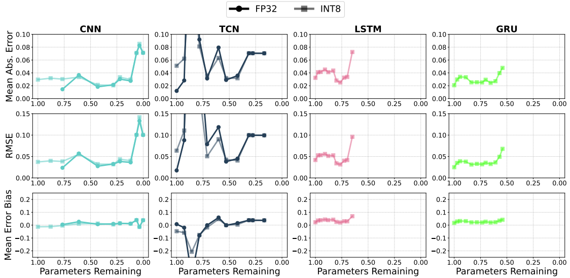
Figure 6: Prediction errors. The less opaque data points denote quantized models. For LSTM and GRU, only the quantized models fit the microcontroller.
