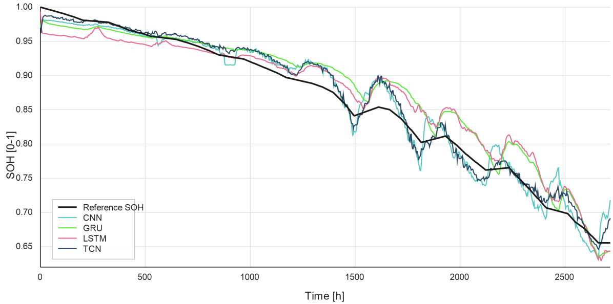
Figure 4: SOH trajectories of the selected uncompressed FP32 baseline models for held-out test cell C11 under continuous causal inference. The black line denotes the reference SOH. For visual clarity, the colored predictions are displayed using a centered seven-hour rolling median, whereas the reported MAE and RMSE values are calculated from the unfiltered predictions.
