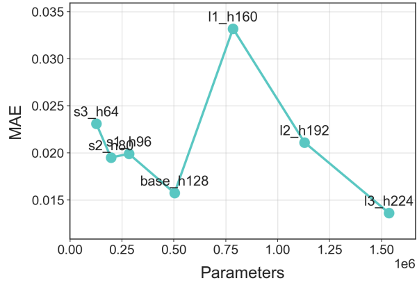
(a) CNN
