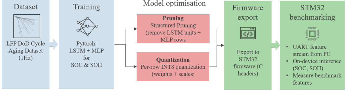
Figure 6.3: End-to-end deployment pipeline from the LFP ageing dataset and PyTorch training to pruning, quantization, C-header export, and final STM32 benchmarking. The same trained SOC and SOH parameter sets form the basis of the floating-point, pruned, and quantized deployments, which keeps the later comparisons numerically consistent.
