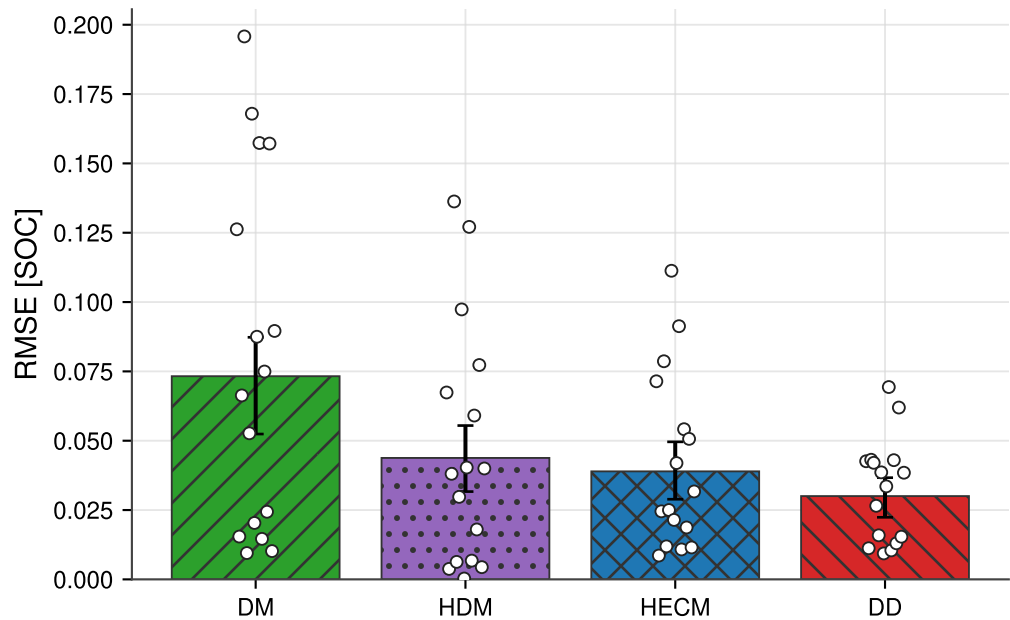
Baseline RMSE
