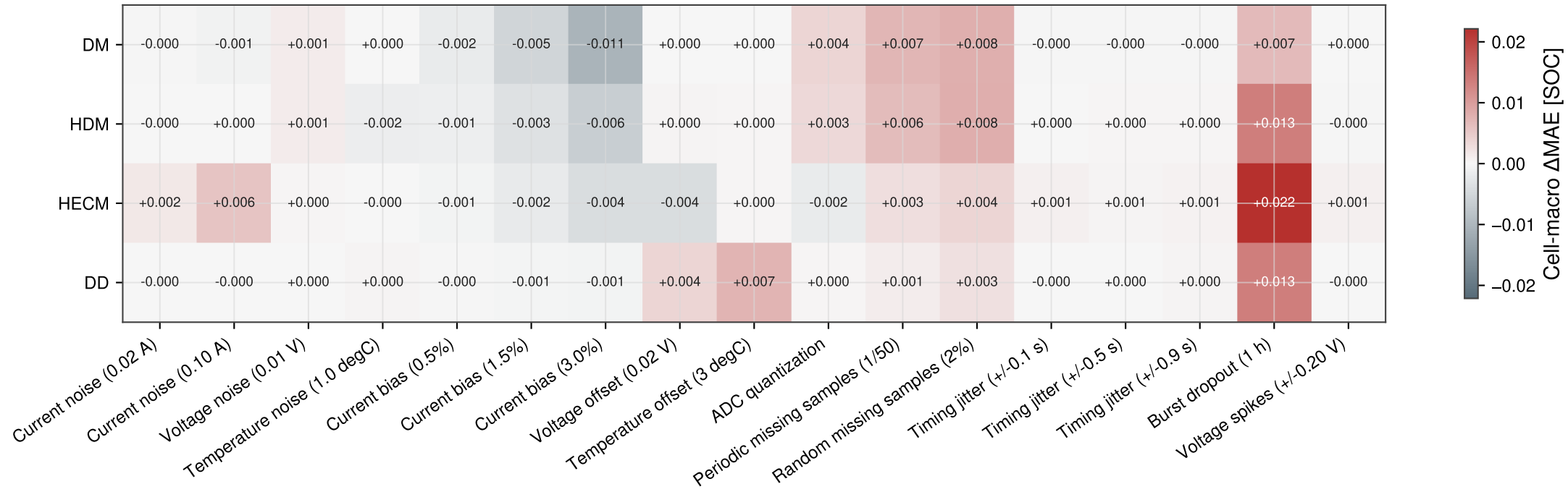
Cross-scenario robustness with independent-cell macro aggregation
