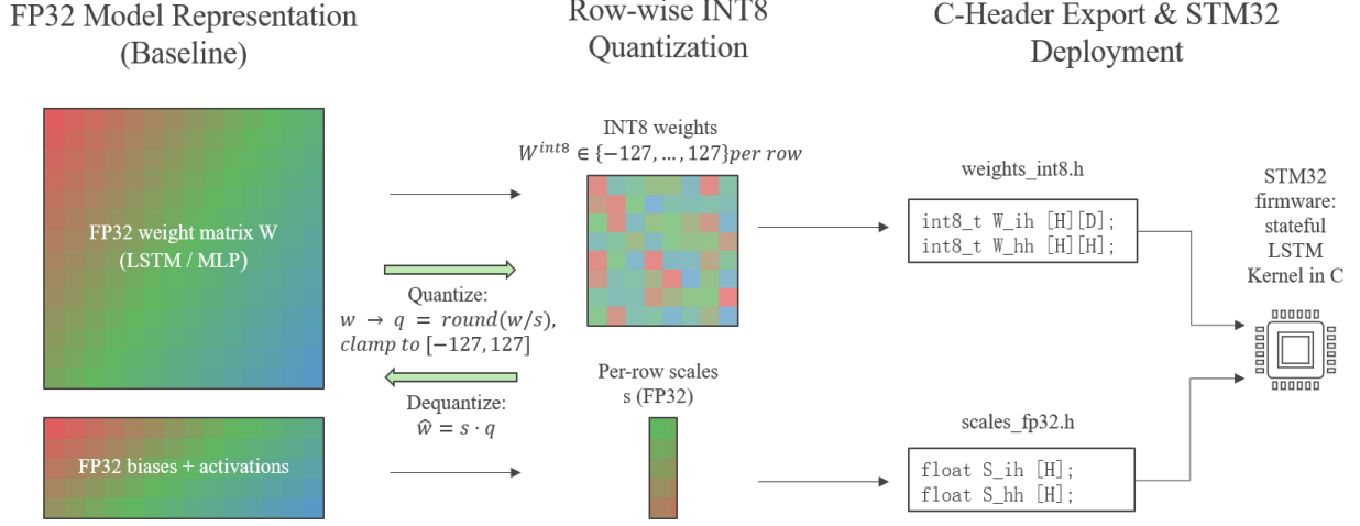
Figure 7: FP32-to-INT8 quantization and embedded deployment. The recurrent FP32 weight matrices are mapped row by row to signed INT8 codes in the symmetric set \{-127, \dots, 127\} together with one FP32 scale per row. The integer recurrent weights and scale vectors are exported as C headers and combined with FP32 biases, activations, recurrent states, and MLP operations in the STM32 kernel.
