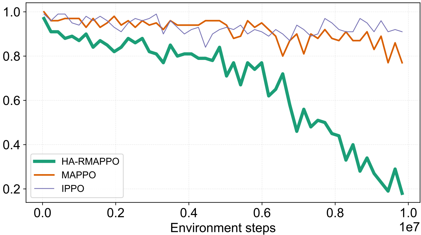
Attack success rate
