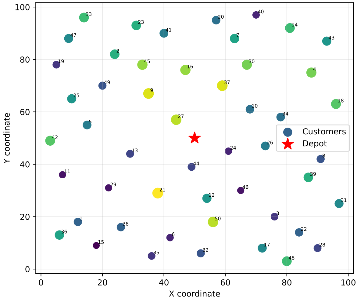
Fixed CVRP Instance
