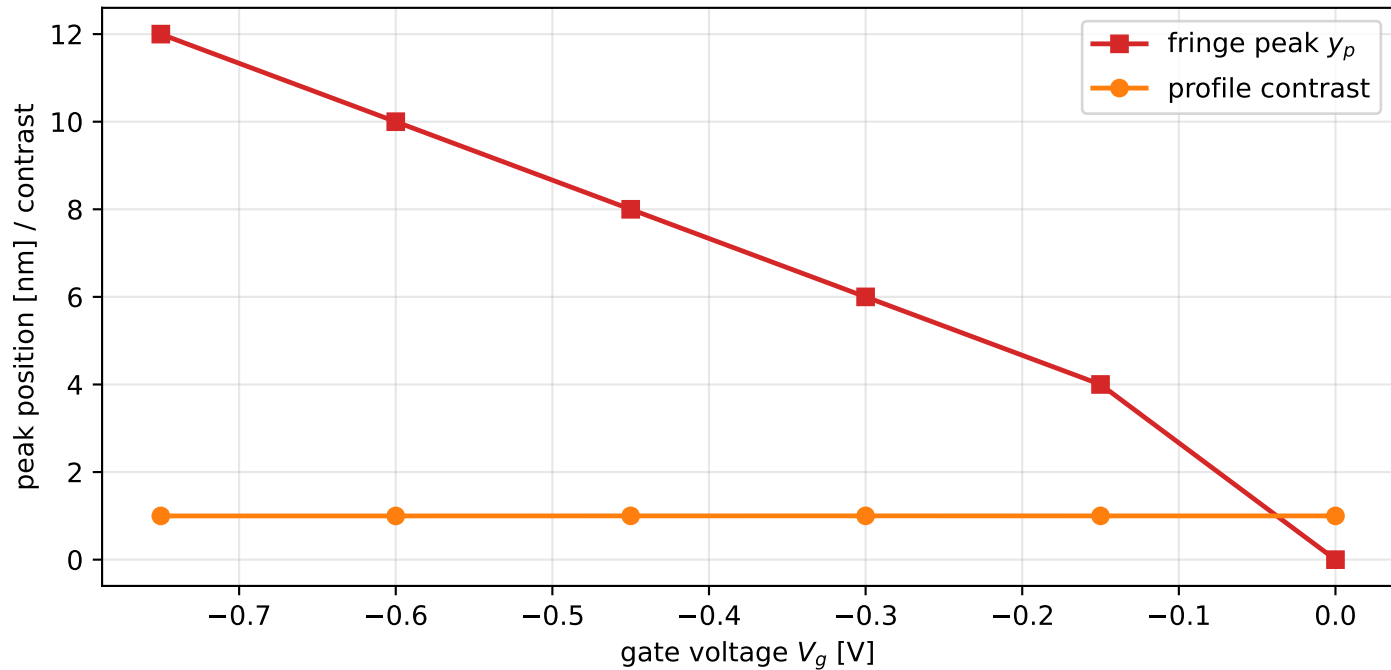
Fringe displacement and contrast vs gate voltage
