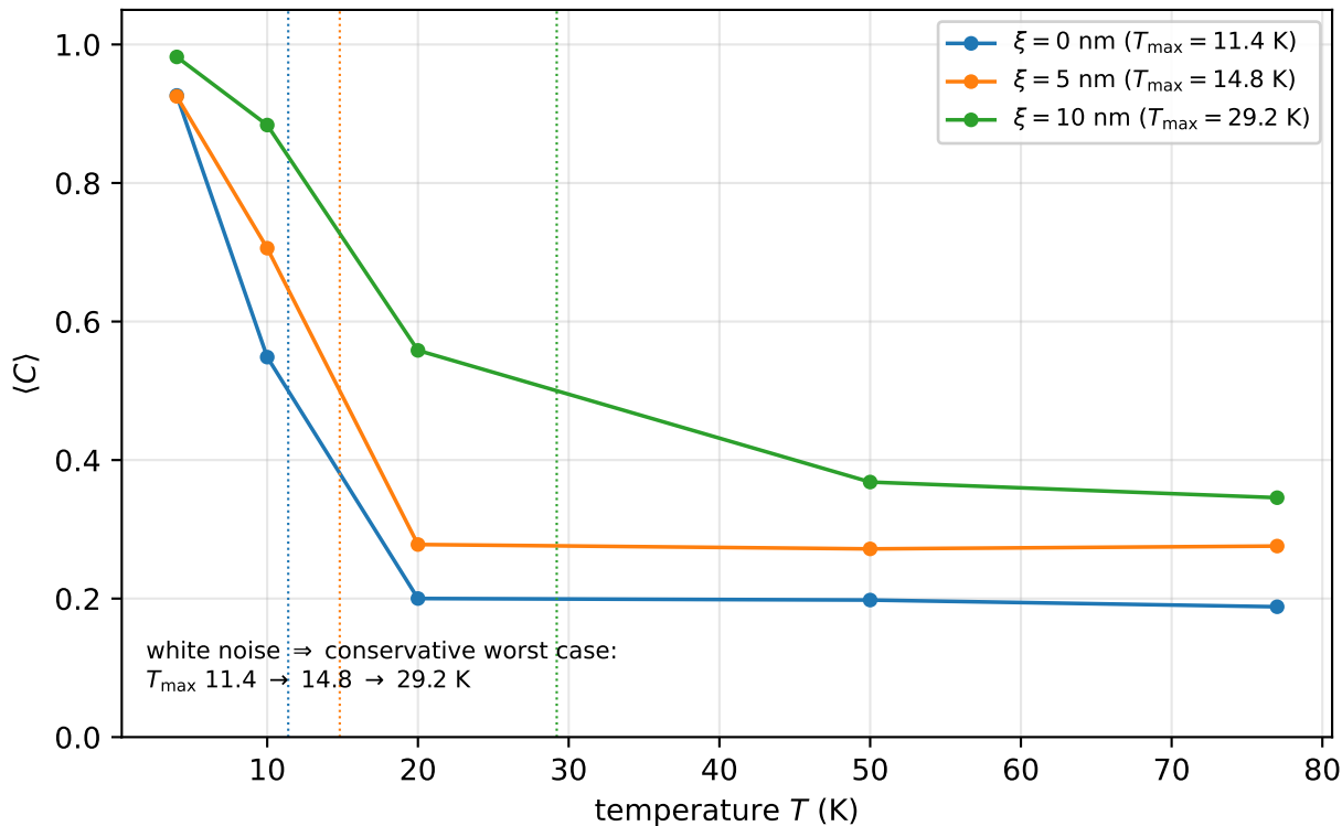
Spatially correlated noise: white noise is the worst case
