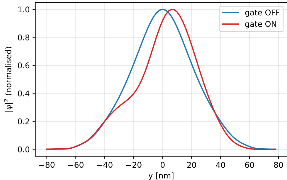
Detector-plane profile: fringe shift by the gate
