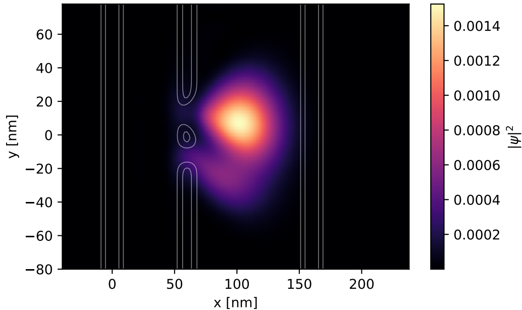
Interference figure, gate ON ( V_\phi on upper slit)
