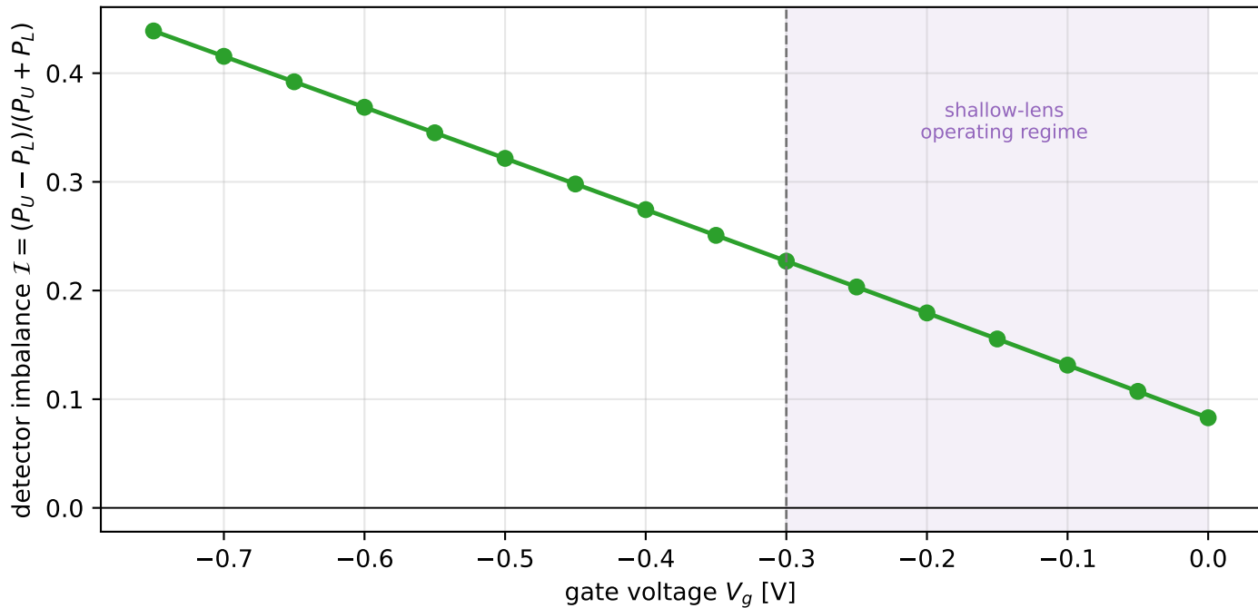
Transfer characteristic: gate-controlled interference logic
