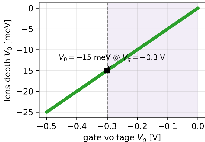
(b) Voltage-to-potential mapping
