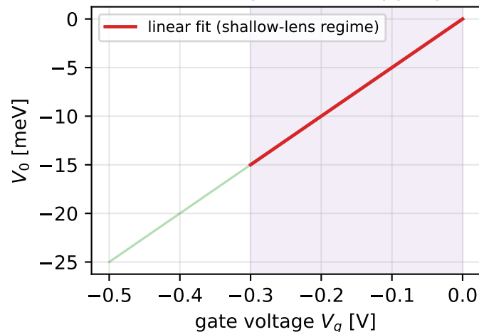
(c) Linearity of the mapping
