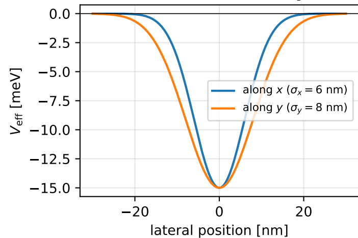
(a) Screened lens profile at V_g = -0.3 V
