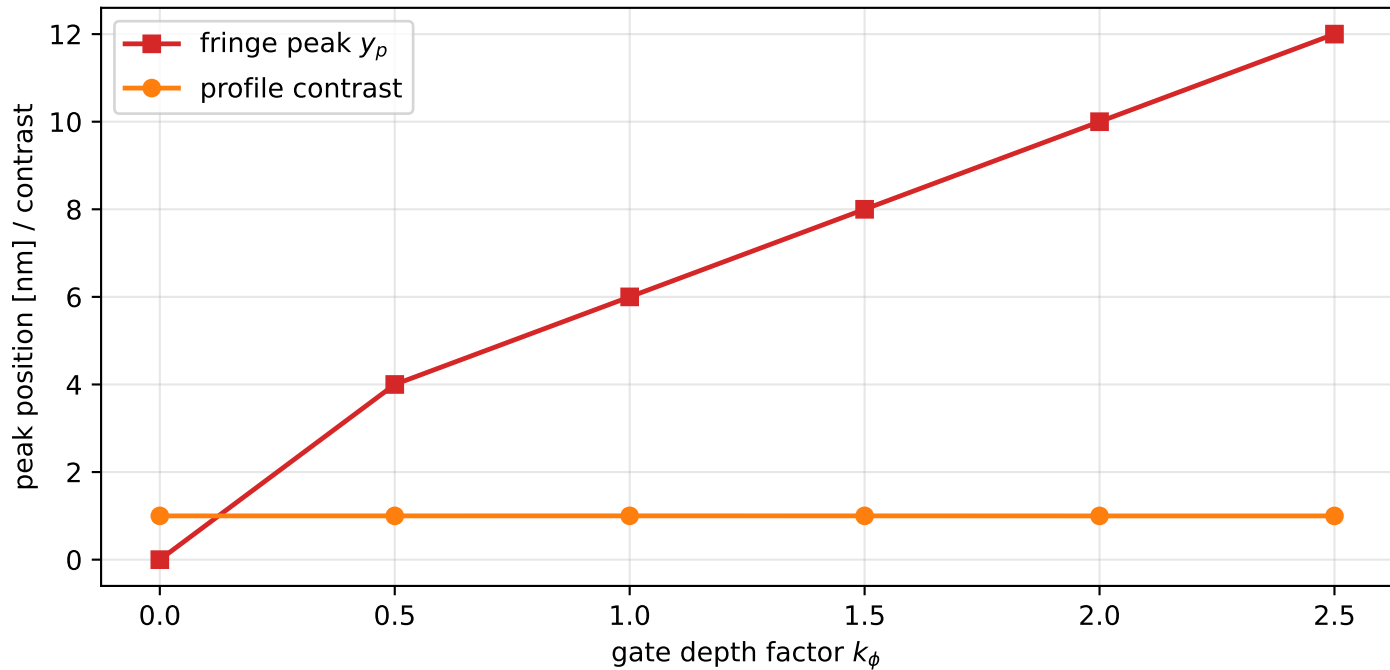
Fringe displacement and contrast vs gate
