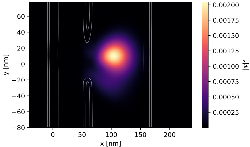
Interference figure, gate ON ( V_\phi on upper slit)
