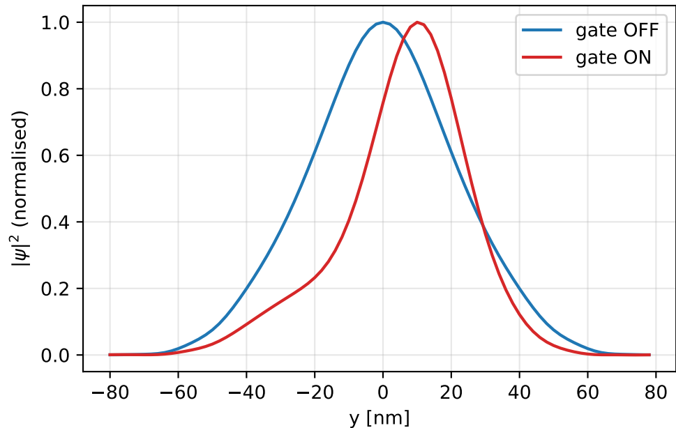
Detector-plane profile: fringe shift by the gate
