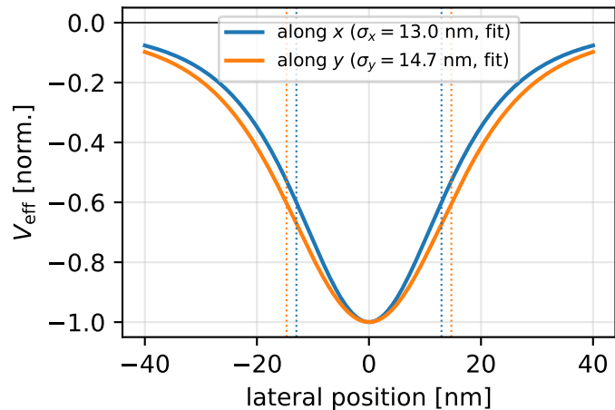
(a) Screened lens profile at V_g = -0.3 \text{ V}
