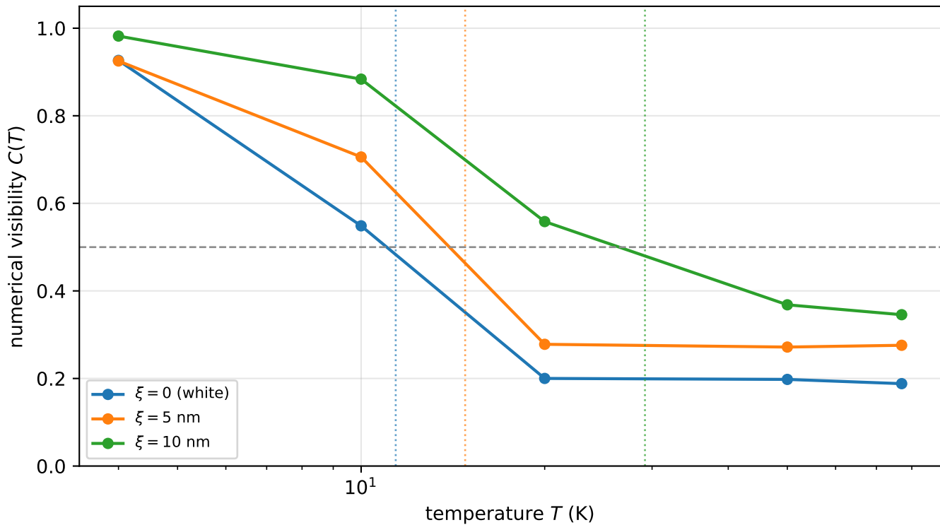
Spatial correlation of the dephasing noise (variance-fixed)
