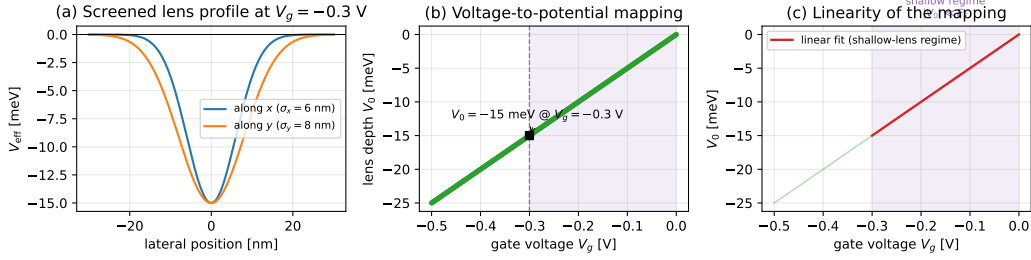
Figure 2: Gate-voltage to effective-potential mapping. (a) Screened effective lens profile V_{\text{eff}} at the operating point V_g = -0.3 V: Gaussian parametrisation of Eq. (5) with V_0 \approx -15 meV, \sigma_x = 6 nm and \sigma_y = 8 nm. (b) Lens depth V_0 vs. V_g : linear in the shallow-lens regime (shaded, |V_g| \leq 0.3 V) with a 50 meV/V coupling. (c) Linear fit in the shallow-lens regime used in the quantum simulations.
