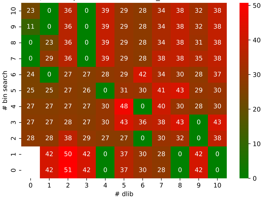
QICE ZFP pressio:abs MAPE: bin_search vs dlib
