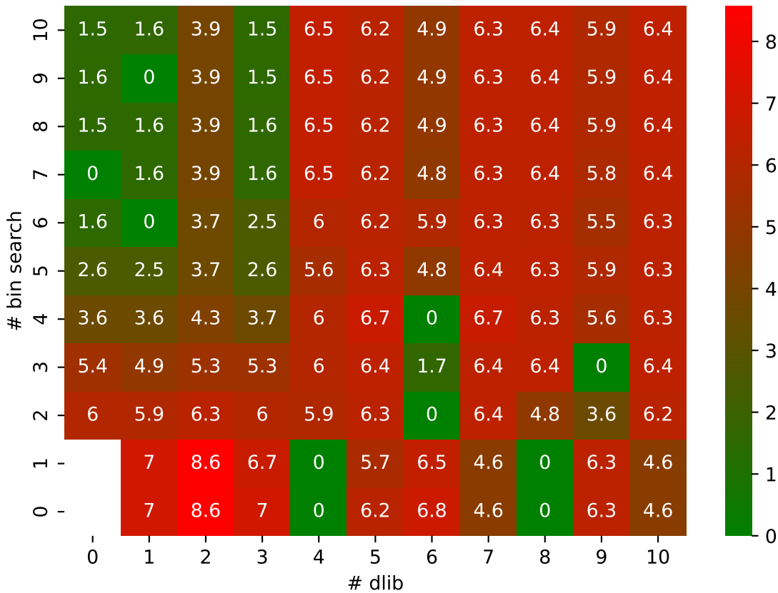
P ZFP pressio:abs MAPE: bin_search vs dlib
