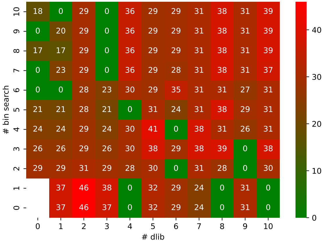
CLOUD ZFP pressio:abs MAPE: bin_search vs dlib
