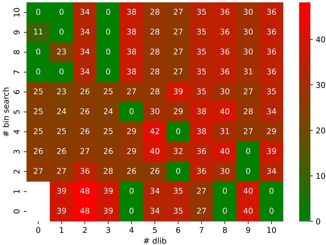
QSNOW ZFP pressio:abs MAPE: bin_search vs dlib
