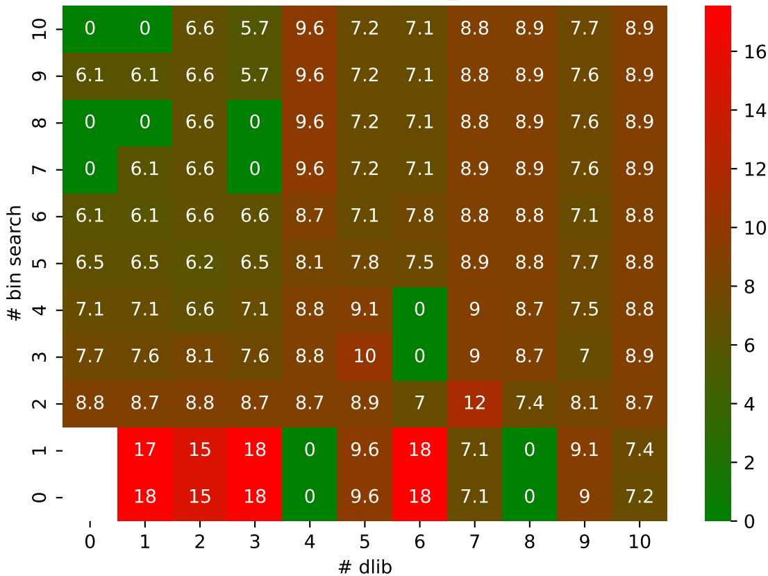
TC ZFP pressio:abs MAPE: bin_search vs dlib
