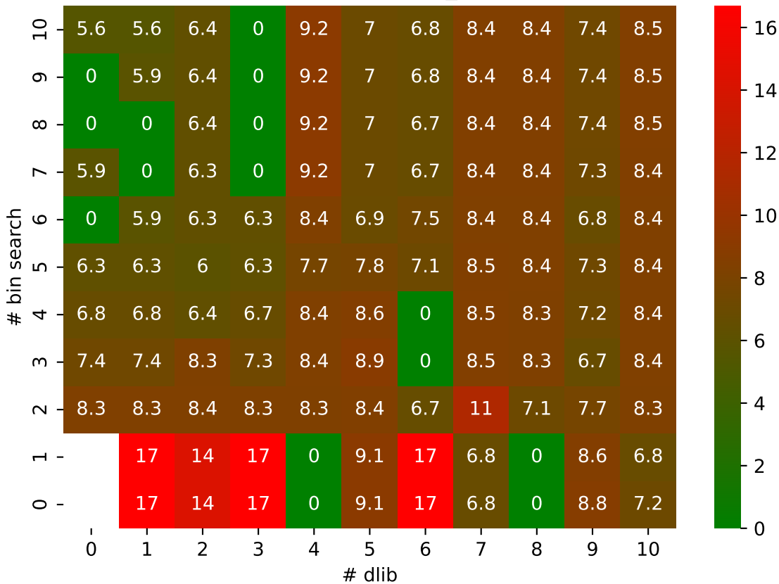
V ZFP pressio:abs MAPE: bin_search vs dlib
