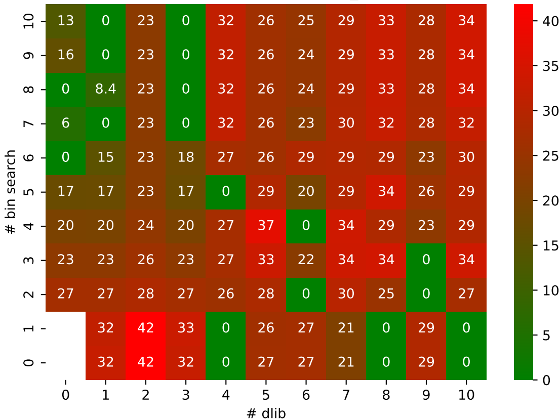
QCLLOUD ZFP pressio:abs MAPE: bin_search vs dlib
