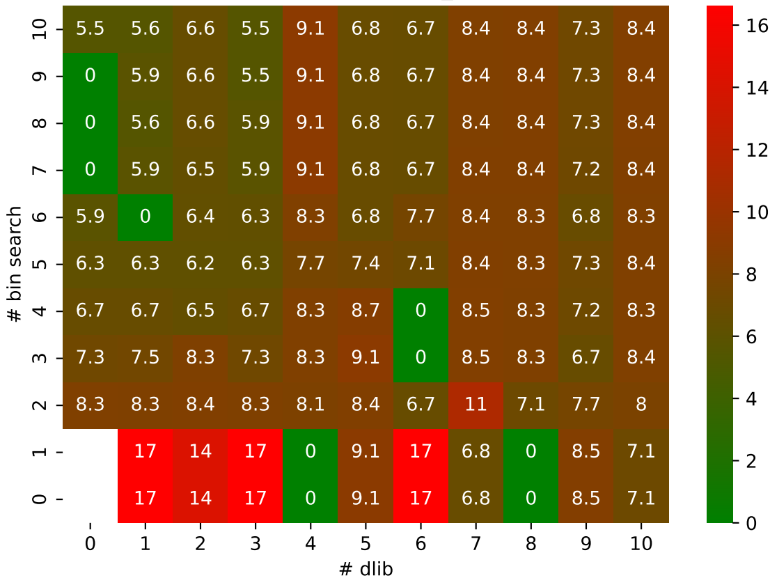
U ZFP pressio:abs MAPE: bin_search vs dlib
