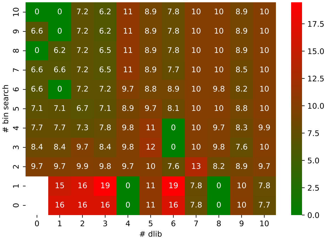
W ZFP pressio:abs MAPE: bin_search vs dlib
