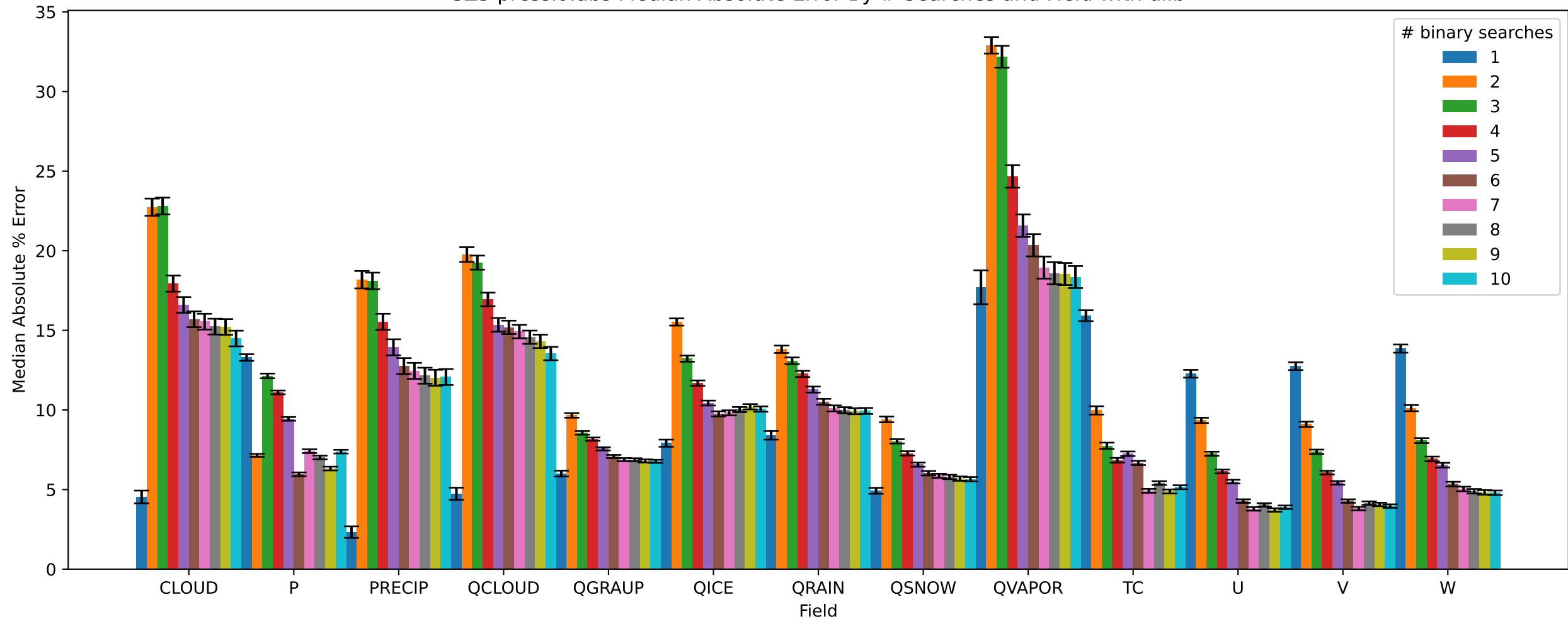
SZ3 pressio:abs Median Absolute Error By # Searches and Field with dlib
