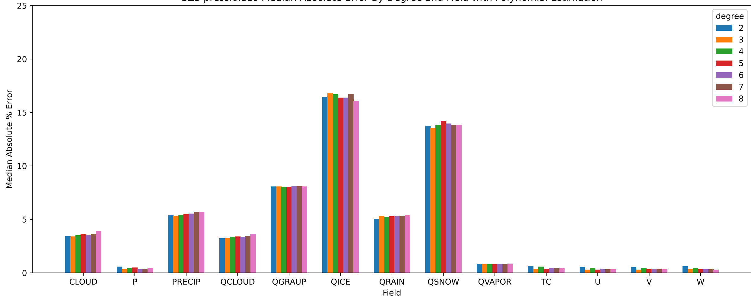
SZ3 pressio:abs Median Absolute Error By Degree and Field with Polynomial Estimation
