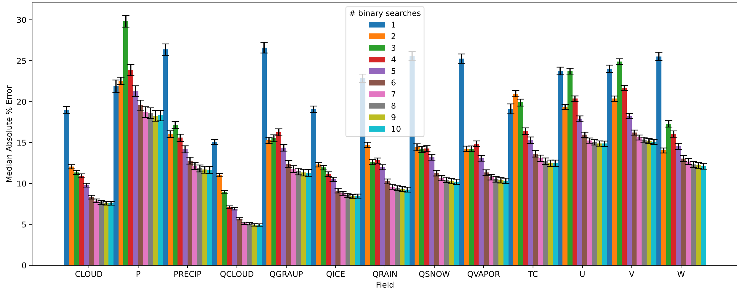
SZ3 pressio:rel Median Absolute Error By # Searches and Field with dlib
