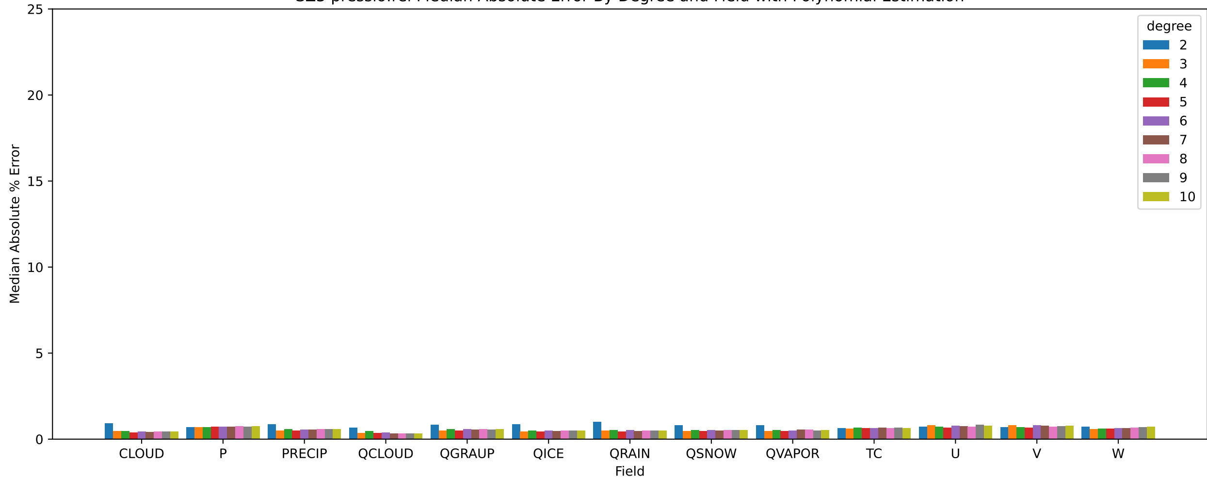
SZ3 pressio:rel Median Absolute Error By Degree and Field with Polynomial Estimation
