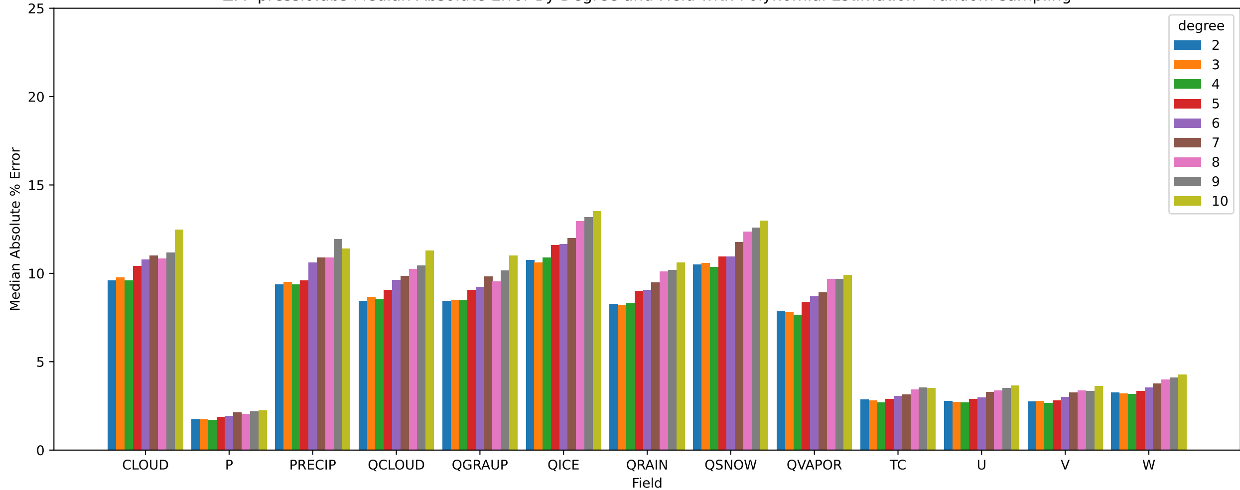
ZFP pressio:abs Median Absolute Error By Degree and Field with Polynomial Estimation - random sampling
