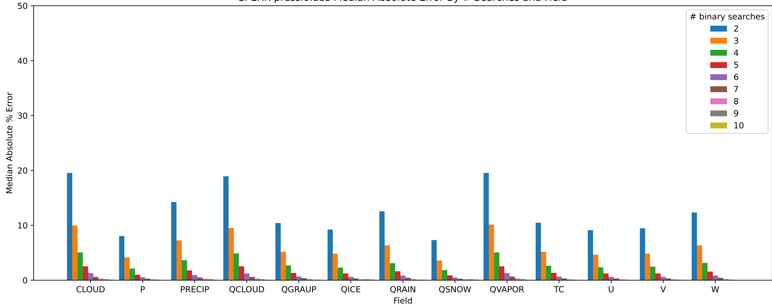
SPERR pressio:abs Median Absolute Error By # Searches and Field
