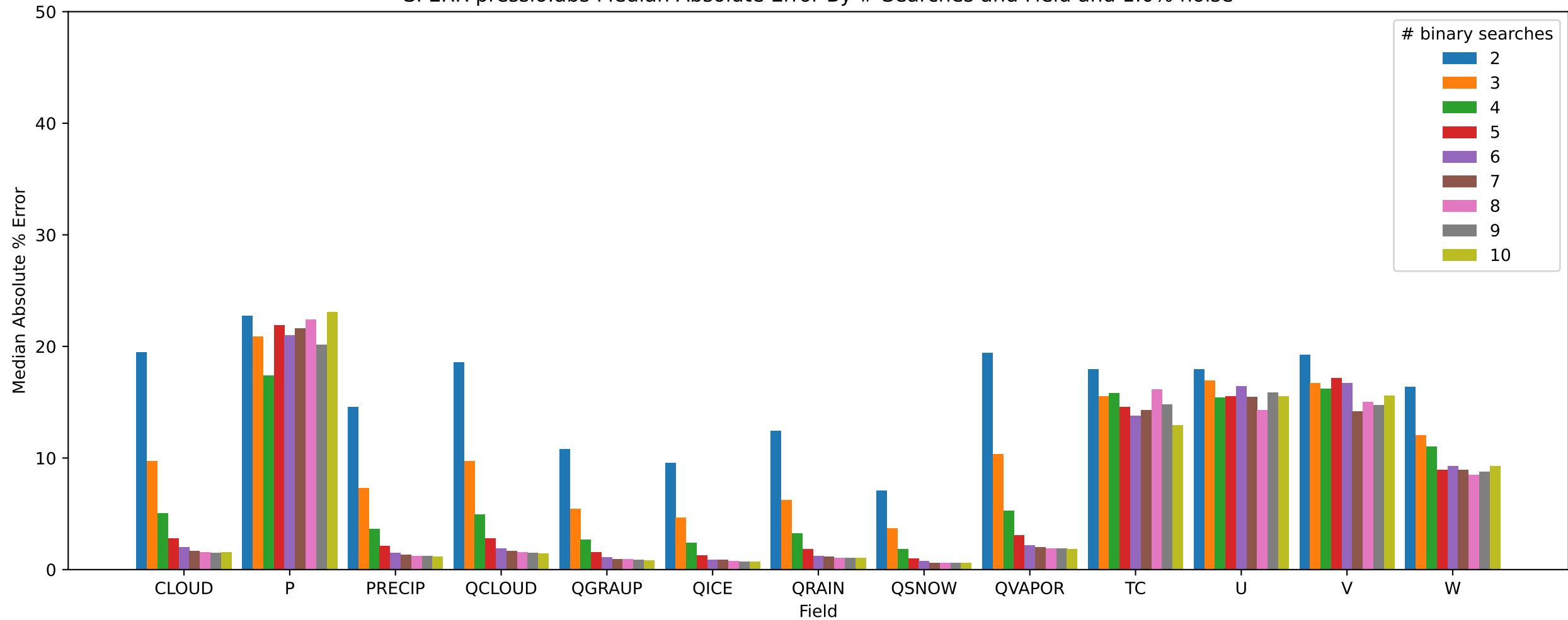
SPERR pressio:abs Median Absolute Error By # Searches and Field and 1.0% noise
