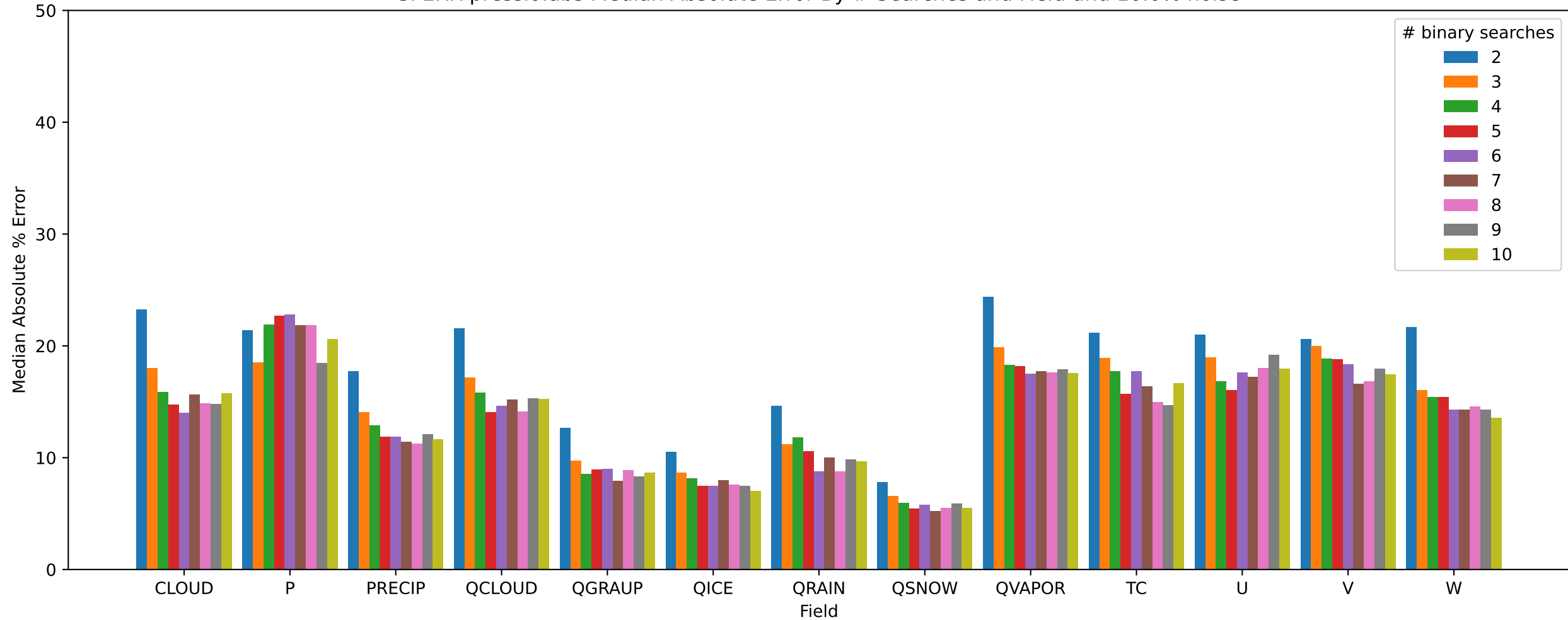
SPERR pressio:abs Median Absolute Error By # Searches and Field and 10.0% noise
