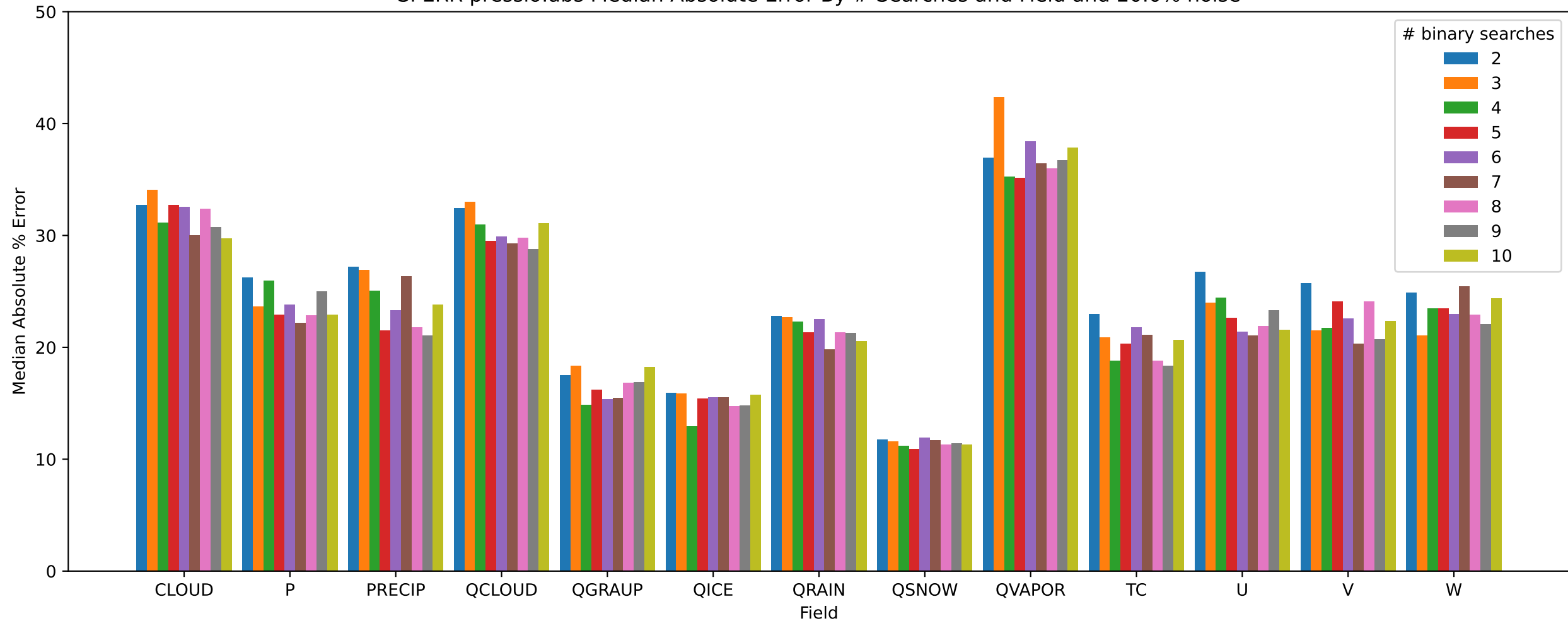
SPERR pressio:abs Median Absolute Error By # Searches and Field and 20.0% noise
