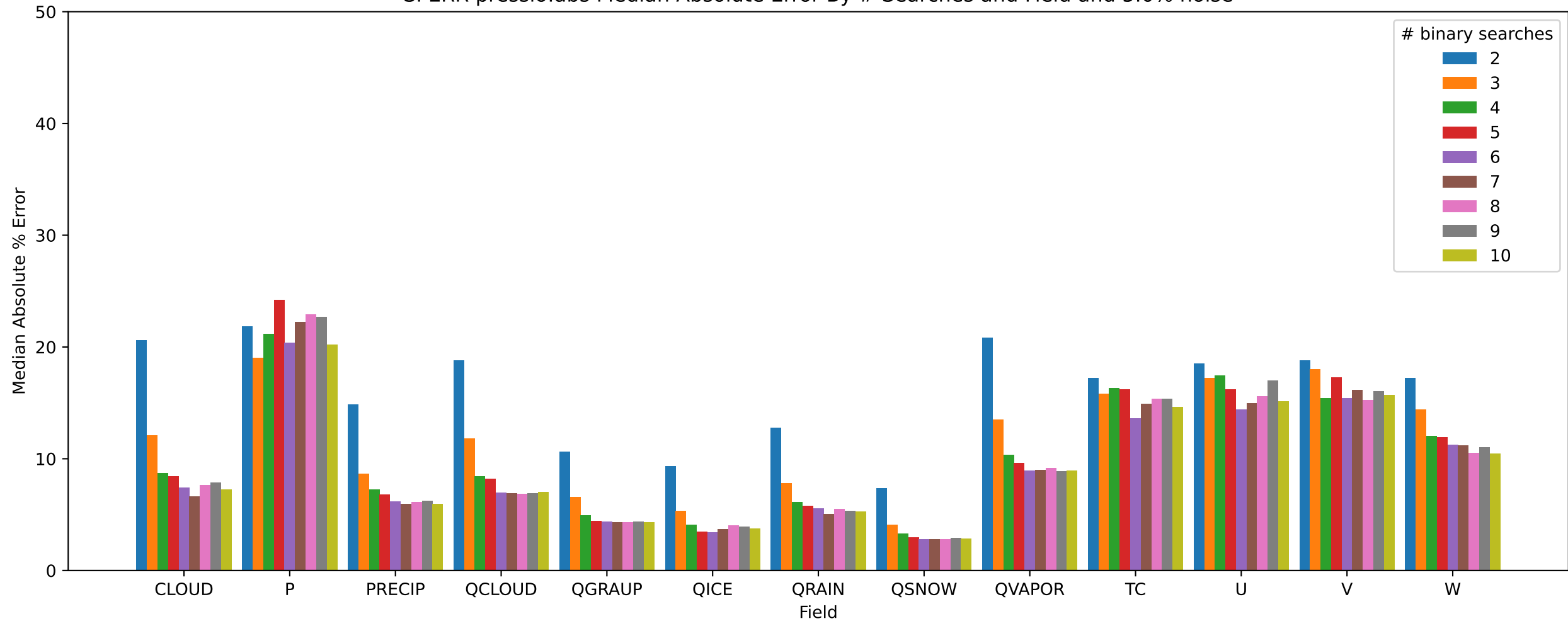
SPERR pressio:abs Median Absolute Error By # Searches and Field and 5.0% noise
