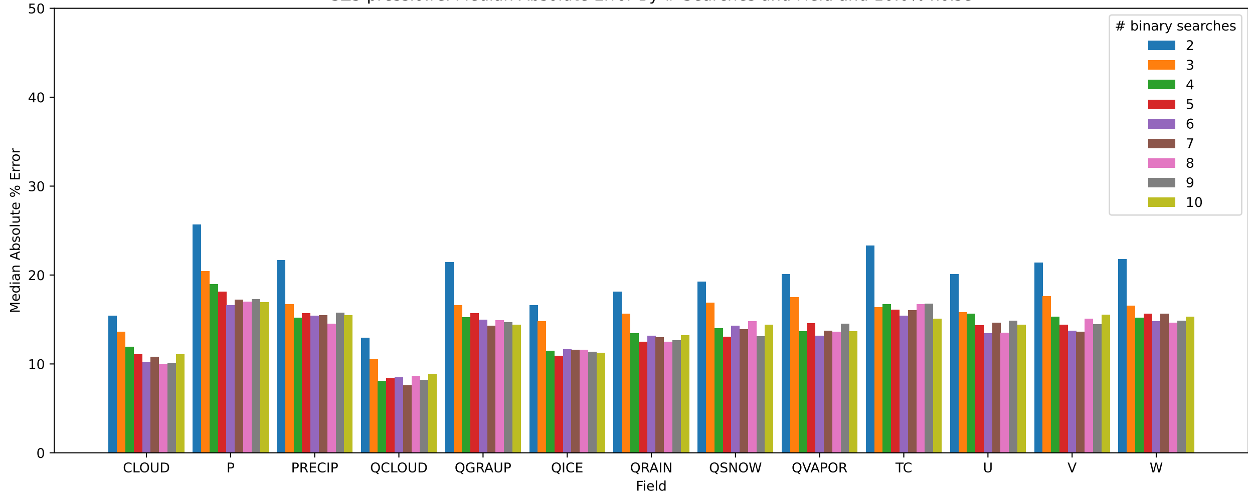
SZ3 pressio:rel Median Absolute Error By # Searches and Field and 10.0% noise
