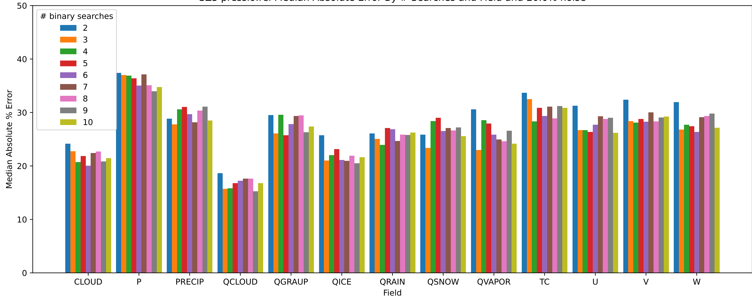
SZ3 pressio:rel Median Absolute Error By # Searches and Field and 20.0% noise
