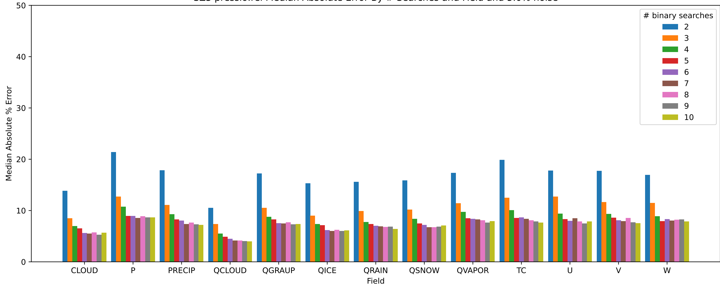
SZ3 pressio:rel Median Absolute Error By # Searches and Field and 5.0% noise
