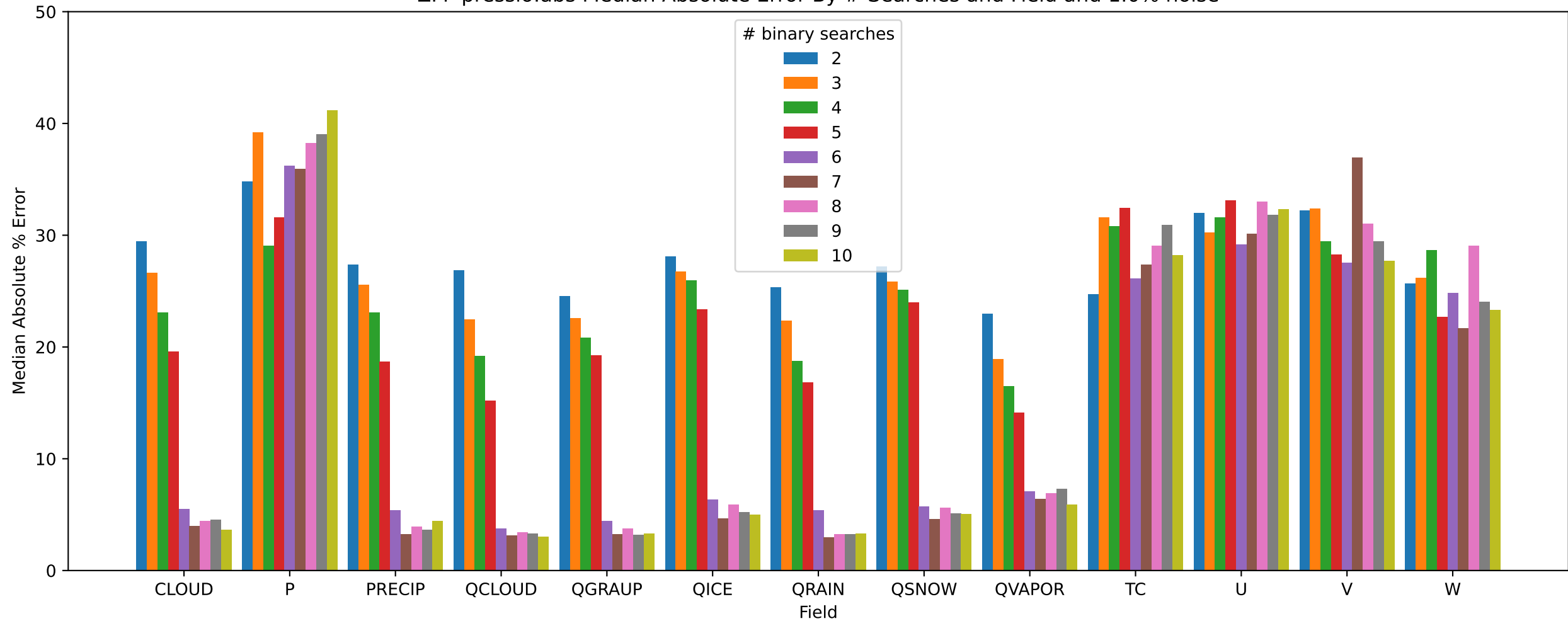
ZFP pressio:abs Median Absolute Error By # Searches and Field and 1.0% noise
