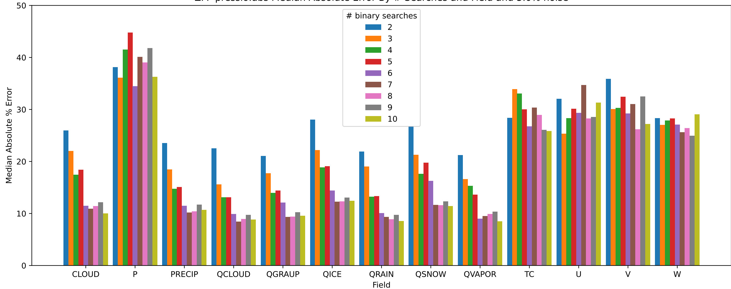
ZFP pressio:abs Median Absolute Error By # Searches and Field and 5.0% noise
