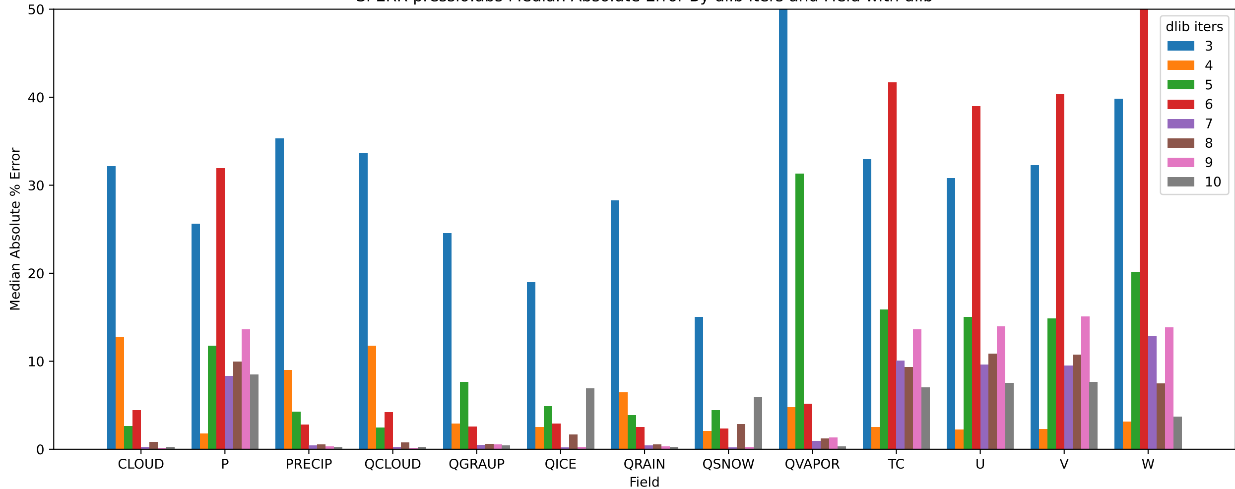
SPERR pressio:abs Median Absolute Error By dlib iters and Field with dlib
