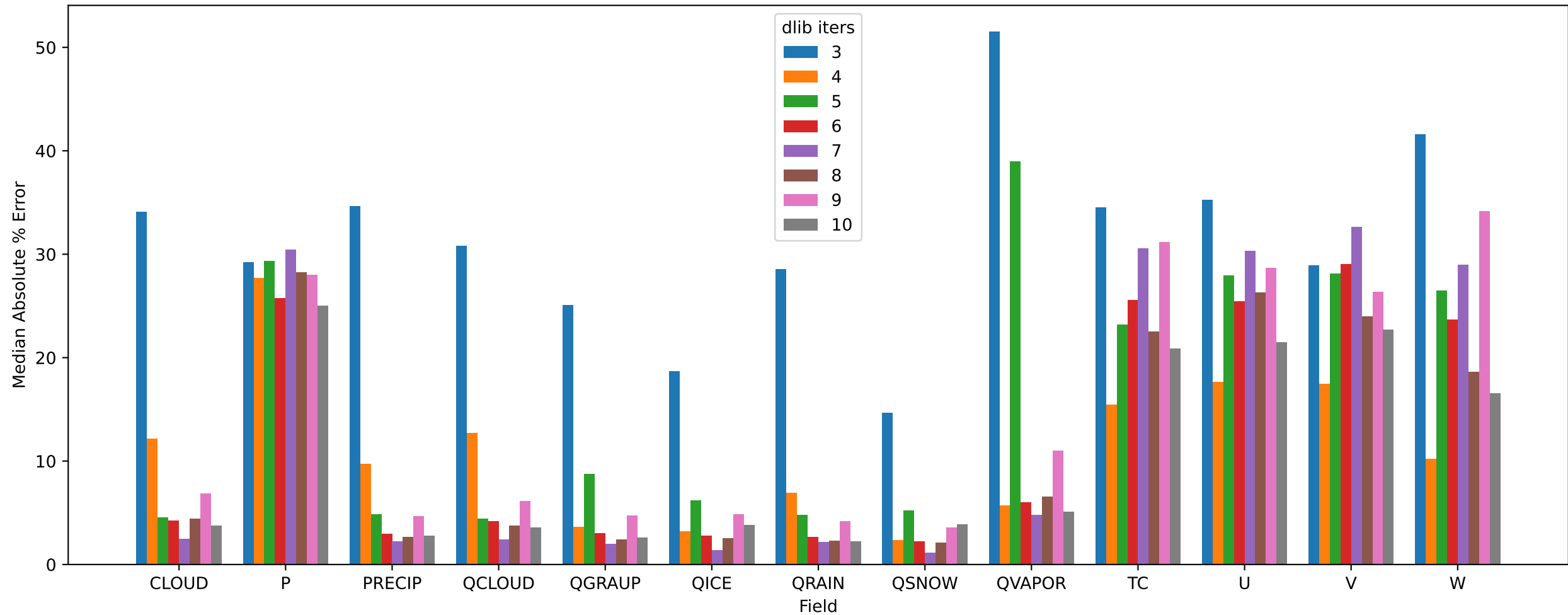
SPERR pressio:abs Median Absolute Error By dlib iters and Field with dlib and 1.0% noise
