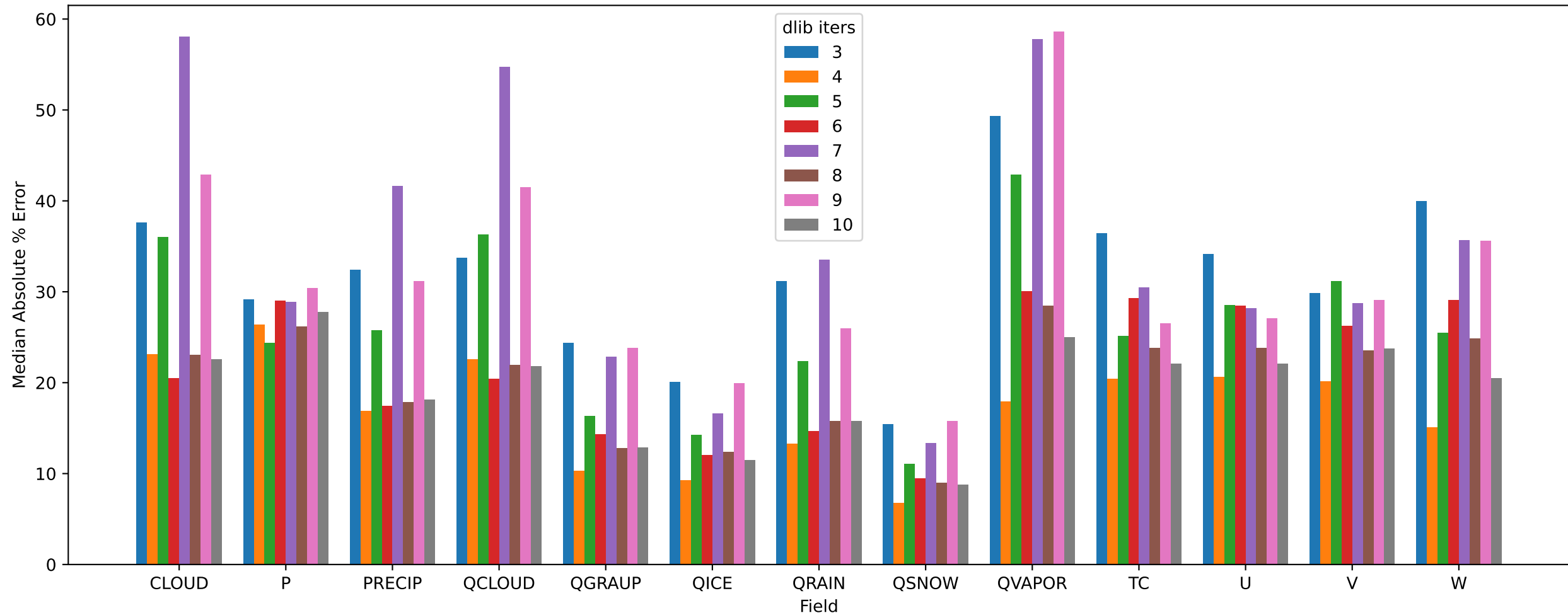
SPERR pressio:abs Median Absolute Error By dlib iters and Field with dlib and 10.0% noise
