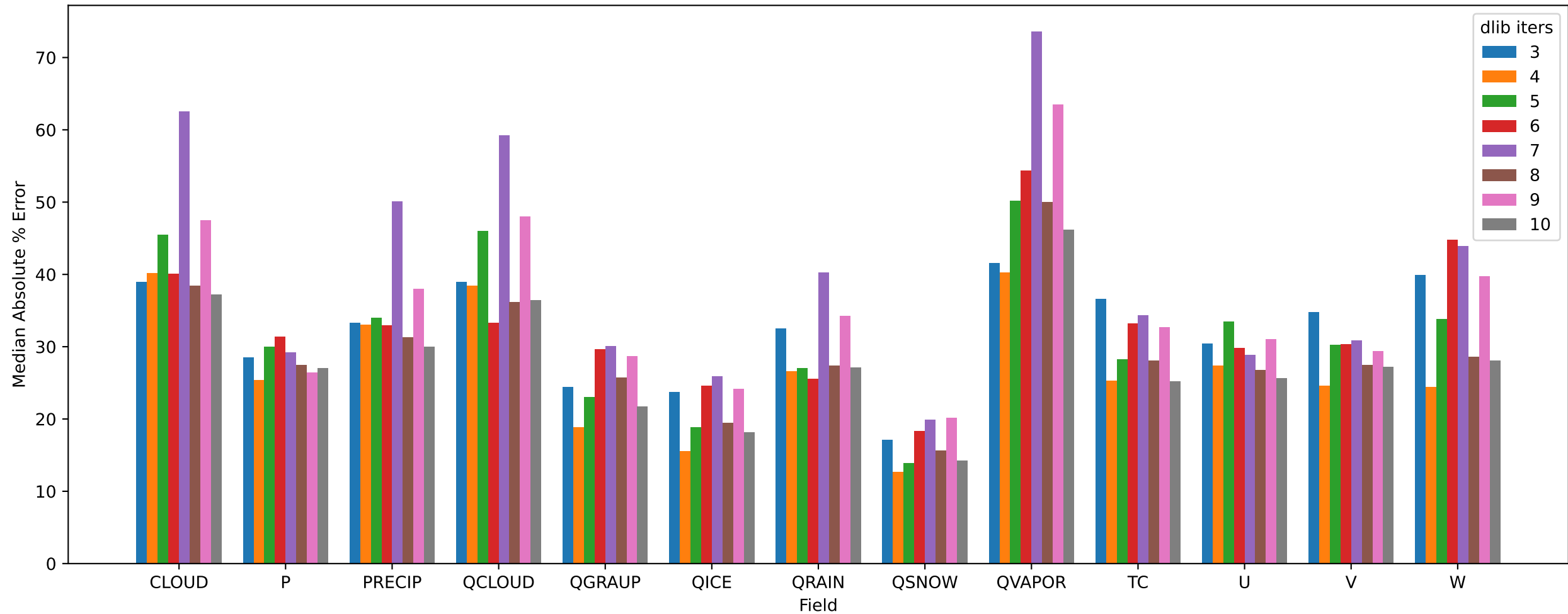
SPERR pressio:abs Median Absolute Error By dlib iters and Field with dlib and 20.0% noise
