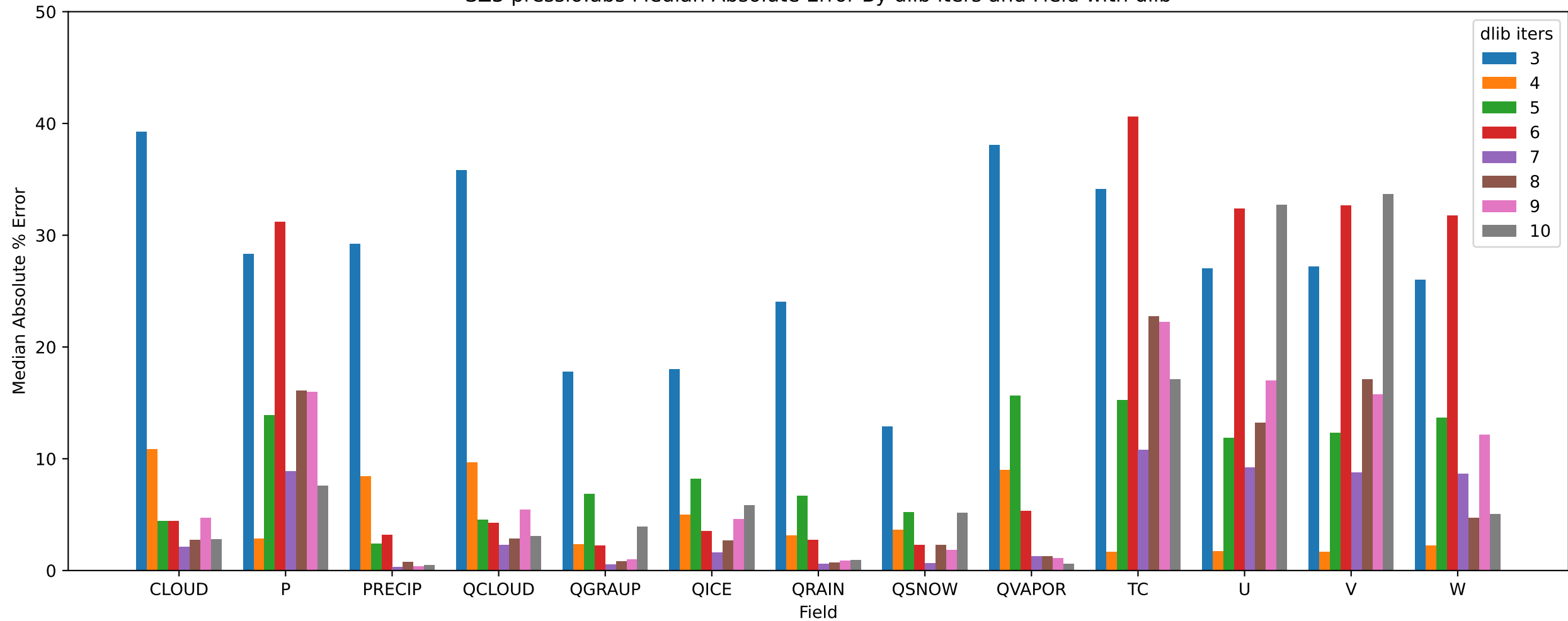
SZ3 pressio:abs Median Absolute Error By dlib iters and Field with dlib
