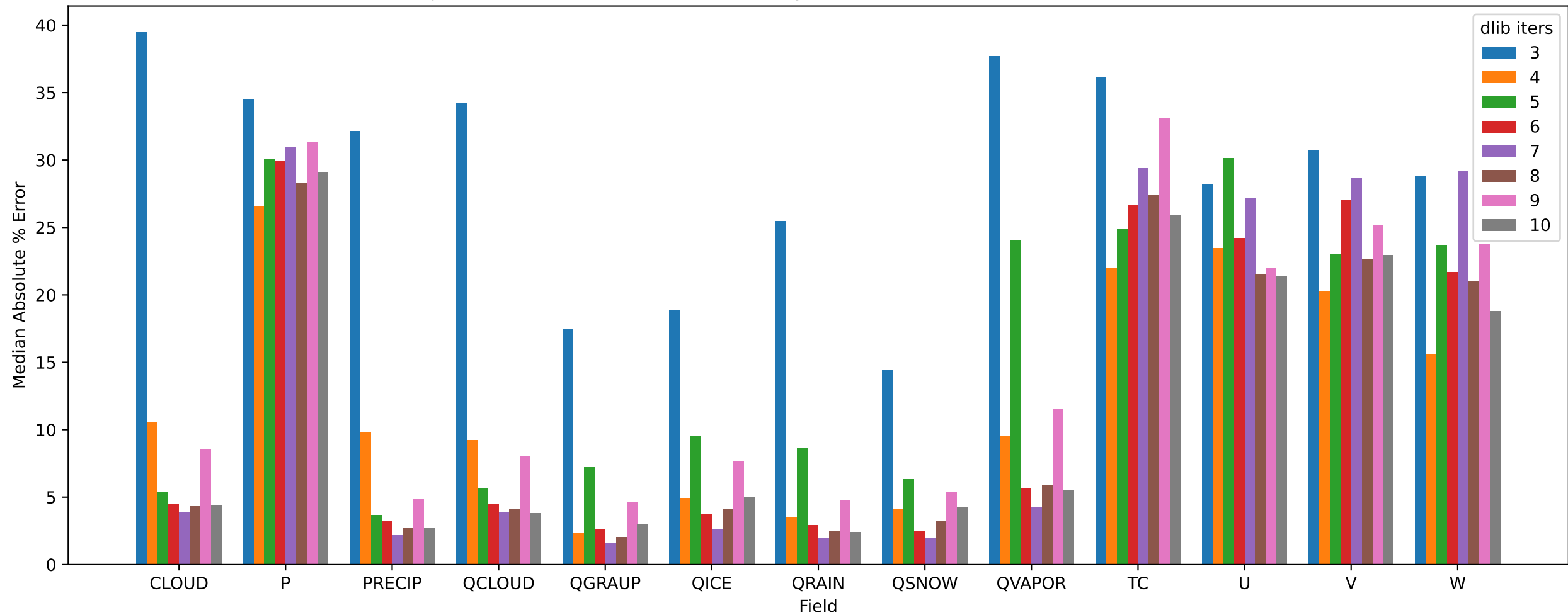
SZ3 pressio:abs Median Absolute Error By dlib iters and Field with dlib and 1.0% noise
