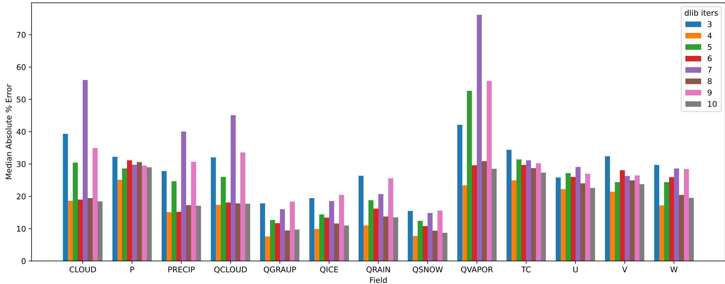
SZ3 pressio:abs Median Absolute Error By dlib iters and Field with dlib and 10.0% noise
