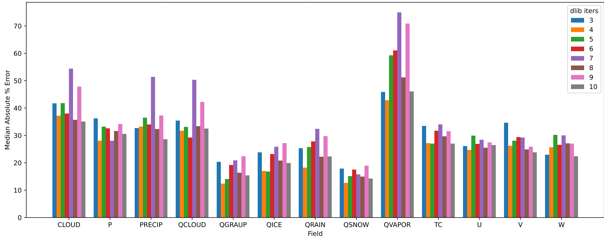
SZ3 pressio:abs Median Absolute Error By dlib iters and Field with dlib and 20.0% noise
