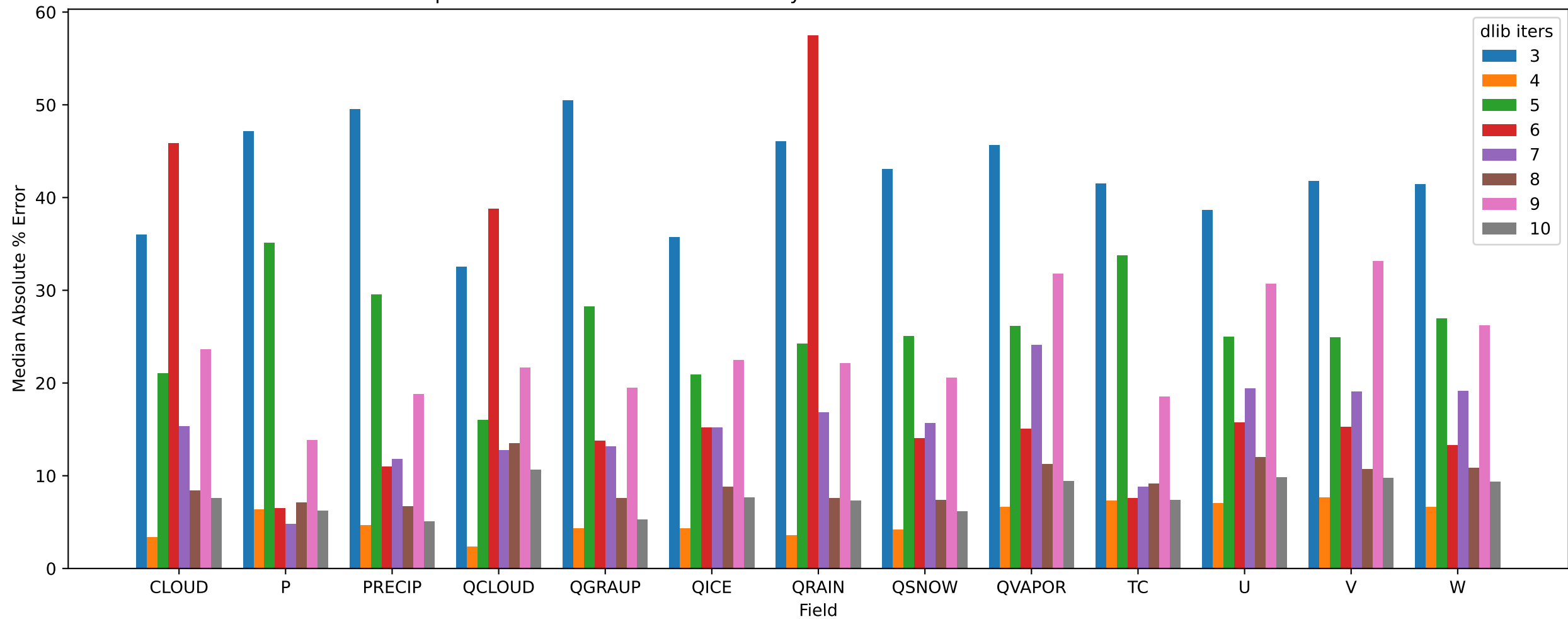
SZ3 pressio:rel Median Absolute Error By dlib iters and Field with dlib and 1.0% noise
