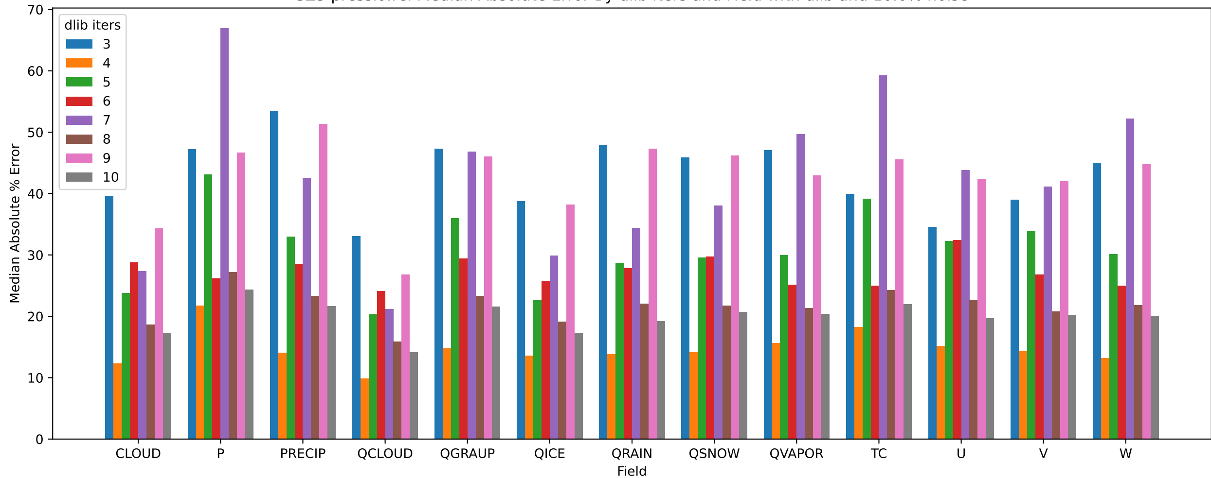
SZ3 pressio:rel Median Absolute Error By dlib iters and Field with dlib and 10.0% noise
