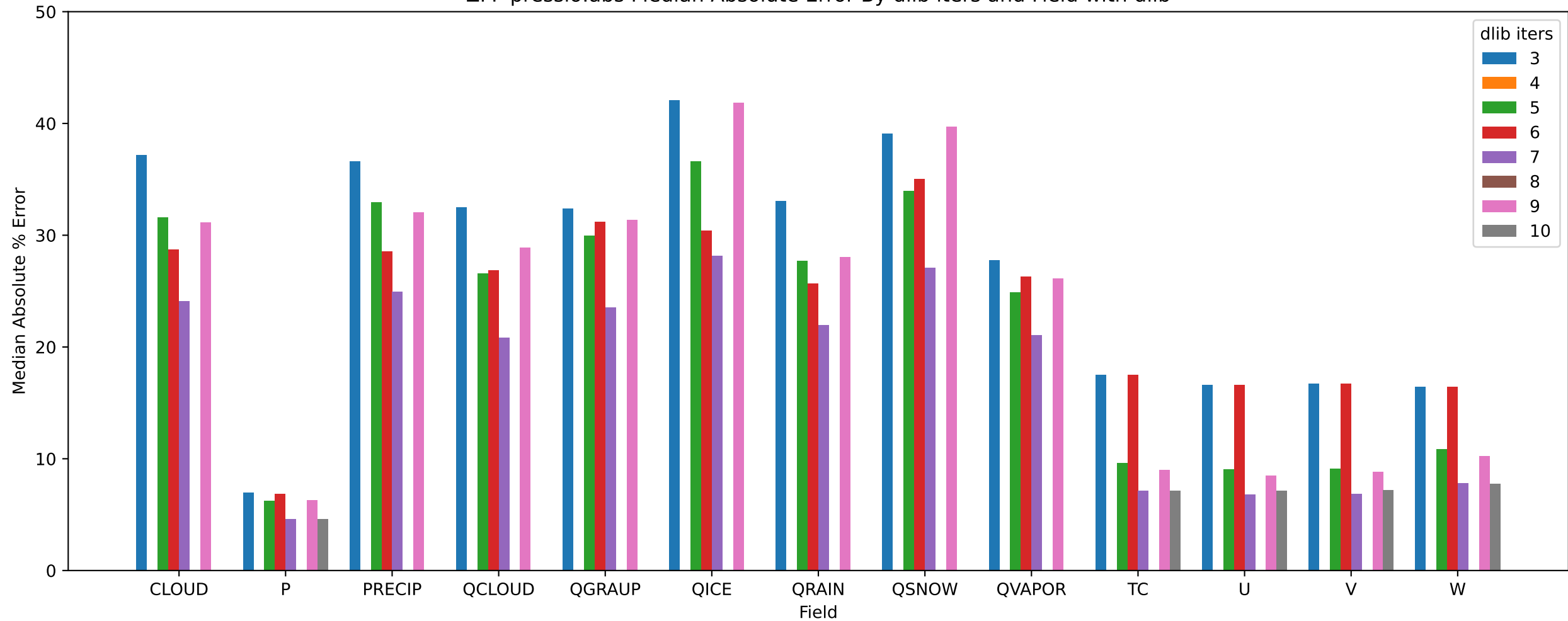
ZFP pressio:abs Median Absolute Error By dlib iters and Field with dlib
