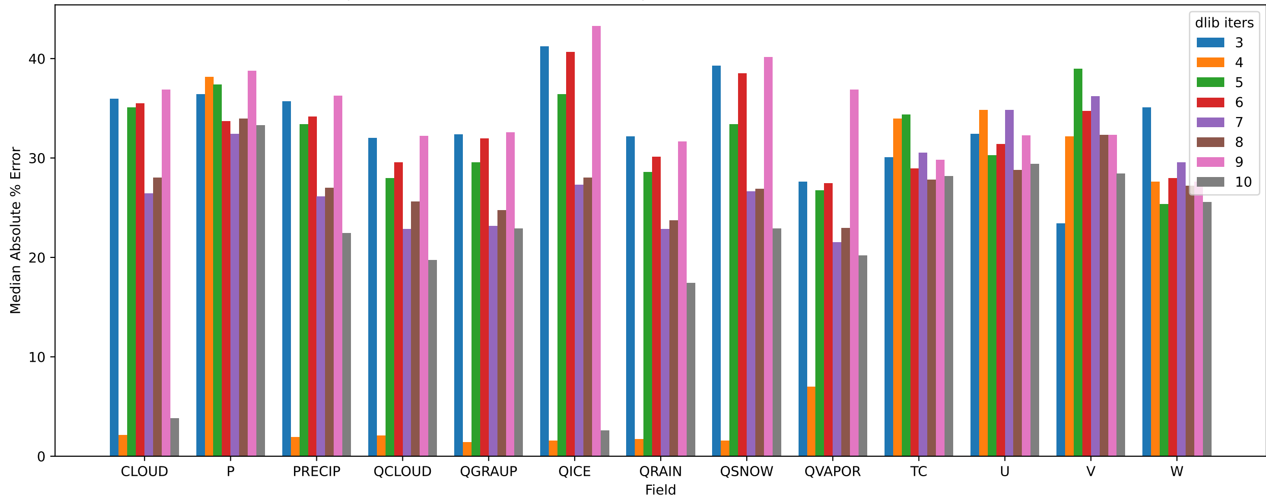
ZFP pressio:abs Median Absolute Error By dlib iters and Field with dlib and 1.0% noise
