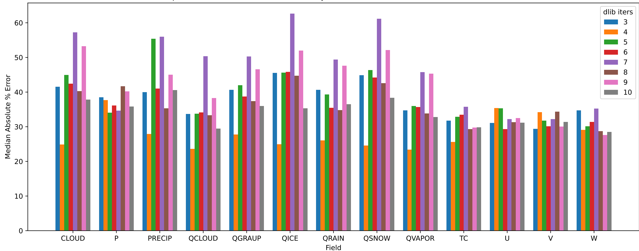
ZFP pressio:abs Median Absolute Error By dlib iters and Field with dlib and 20.0% noise
