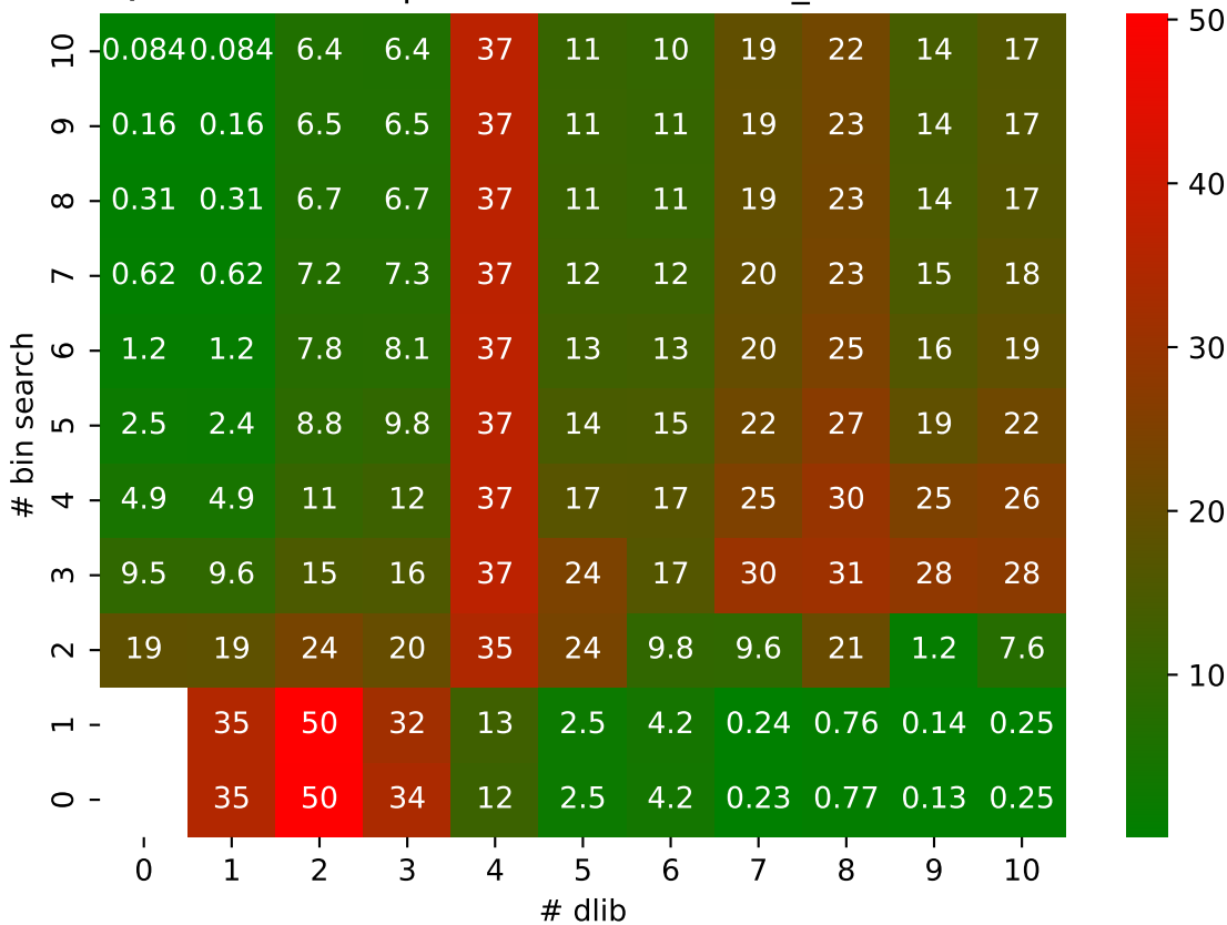
QCCLOUD SPERR pressio:abs MAPE: bin_search vs dlib
