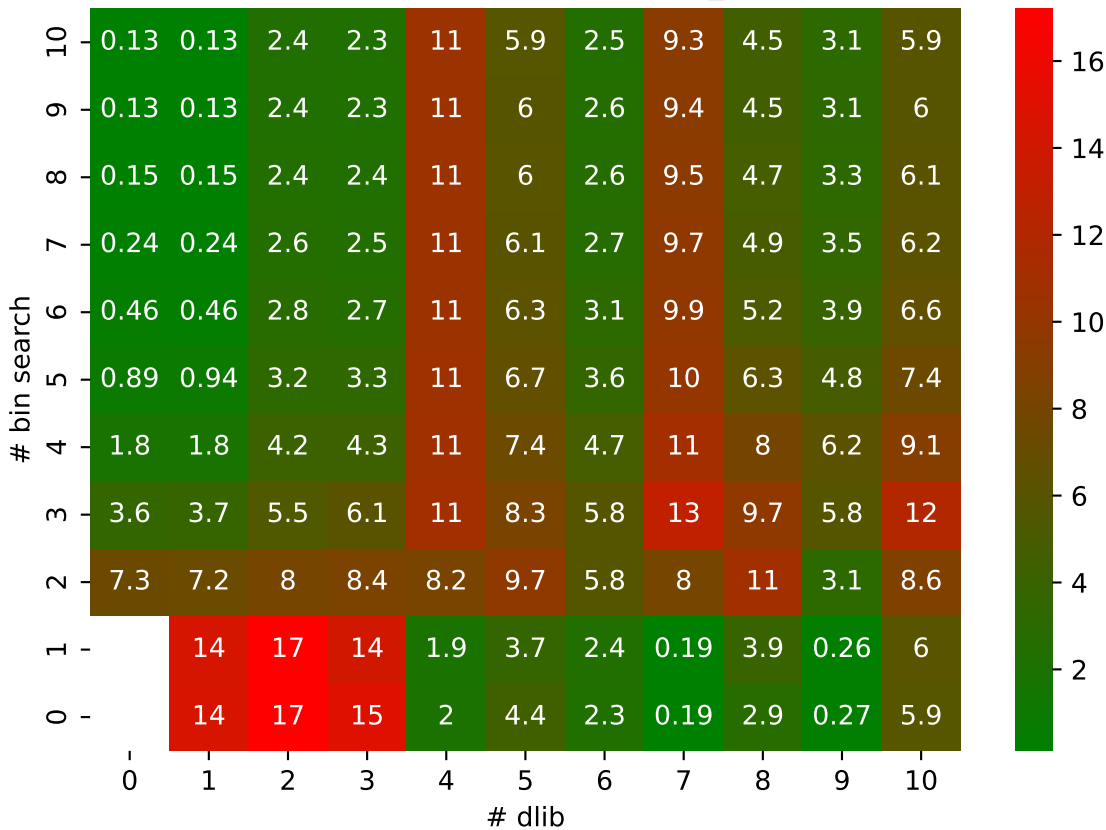
QSNOW SPERR pressio:abs MAPE: bin_search vs dlib
