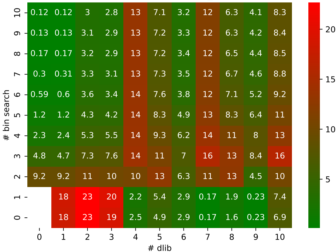
QICE SPERR pressio:abs MAPE: bin_search vs dlib
