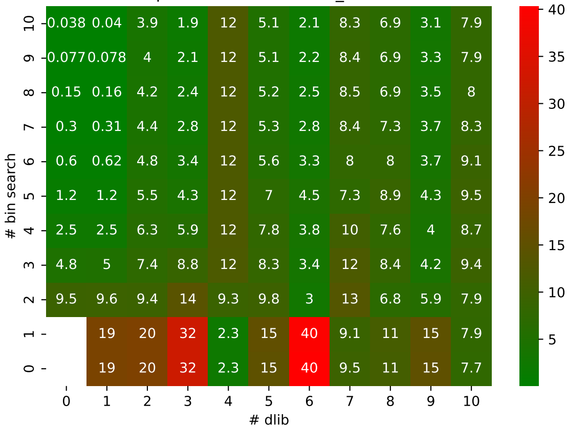
V SPERR pressio:abs MAPE: bin_search vs dlib
