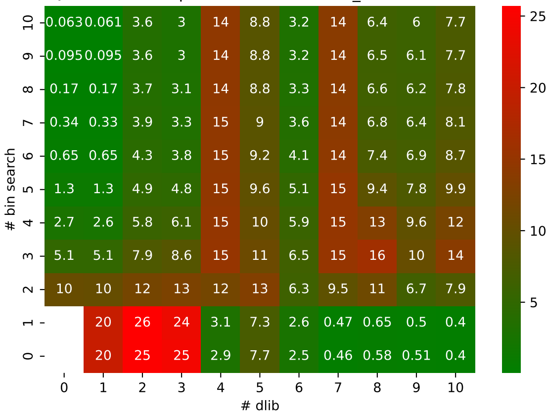
QGRAUP SPERR pressio:abs MAPE: bin_search vs dlib
