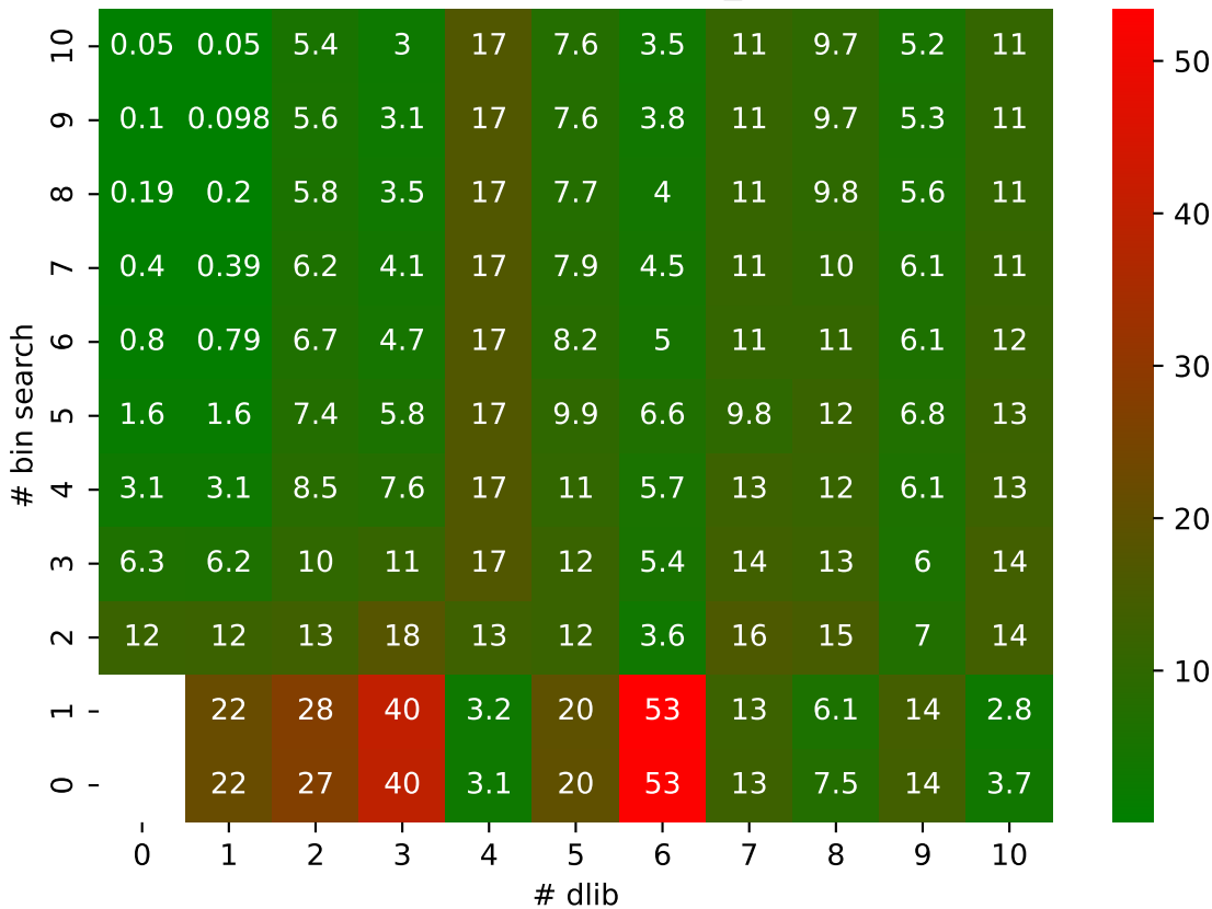
W SPERR pressio:abs MAPE: bin_search vs dlib
