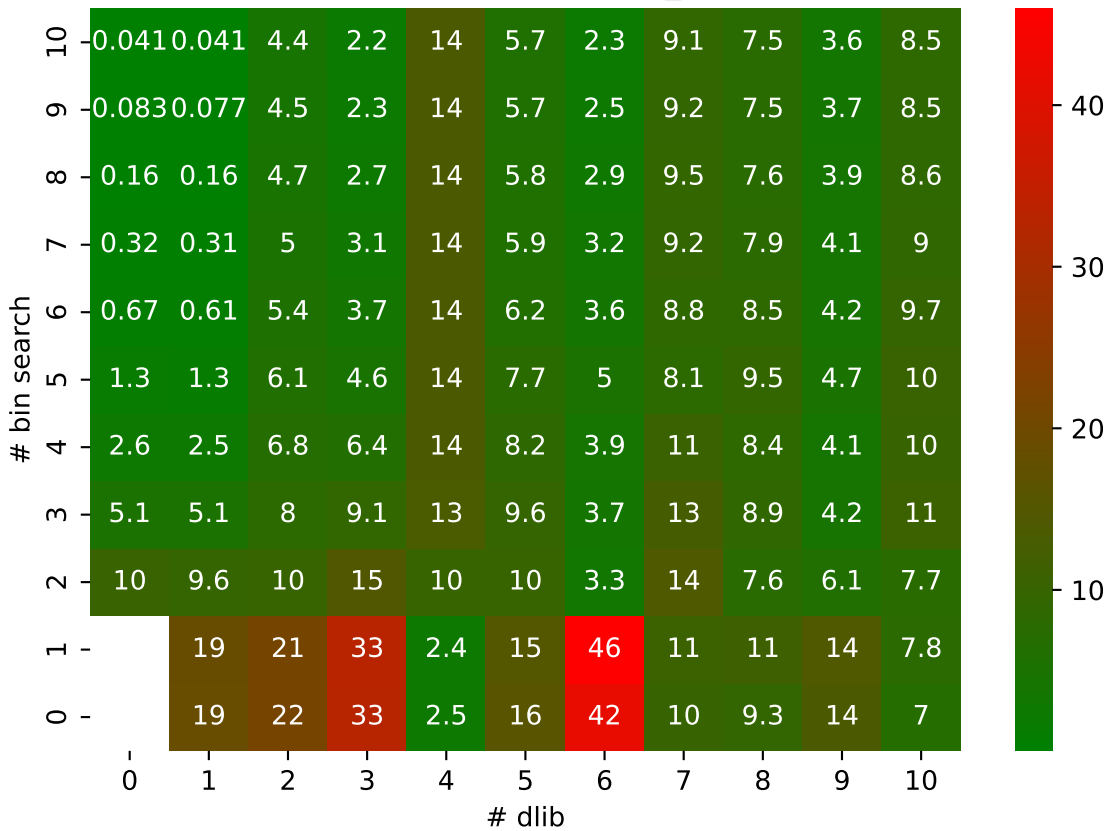
TC SPERR pressio:abs MAPE: bin_search vs dlib
