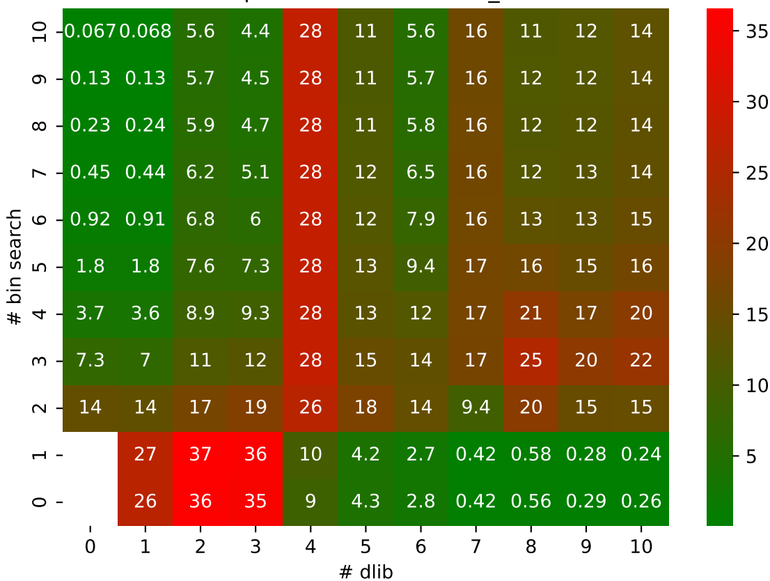
PRECIP SPERR pressio:abs MAPE: bin_search vs dlib
