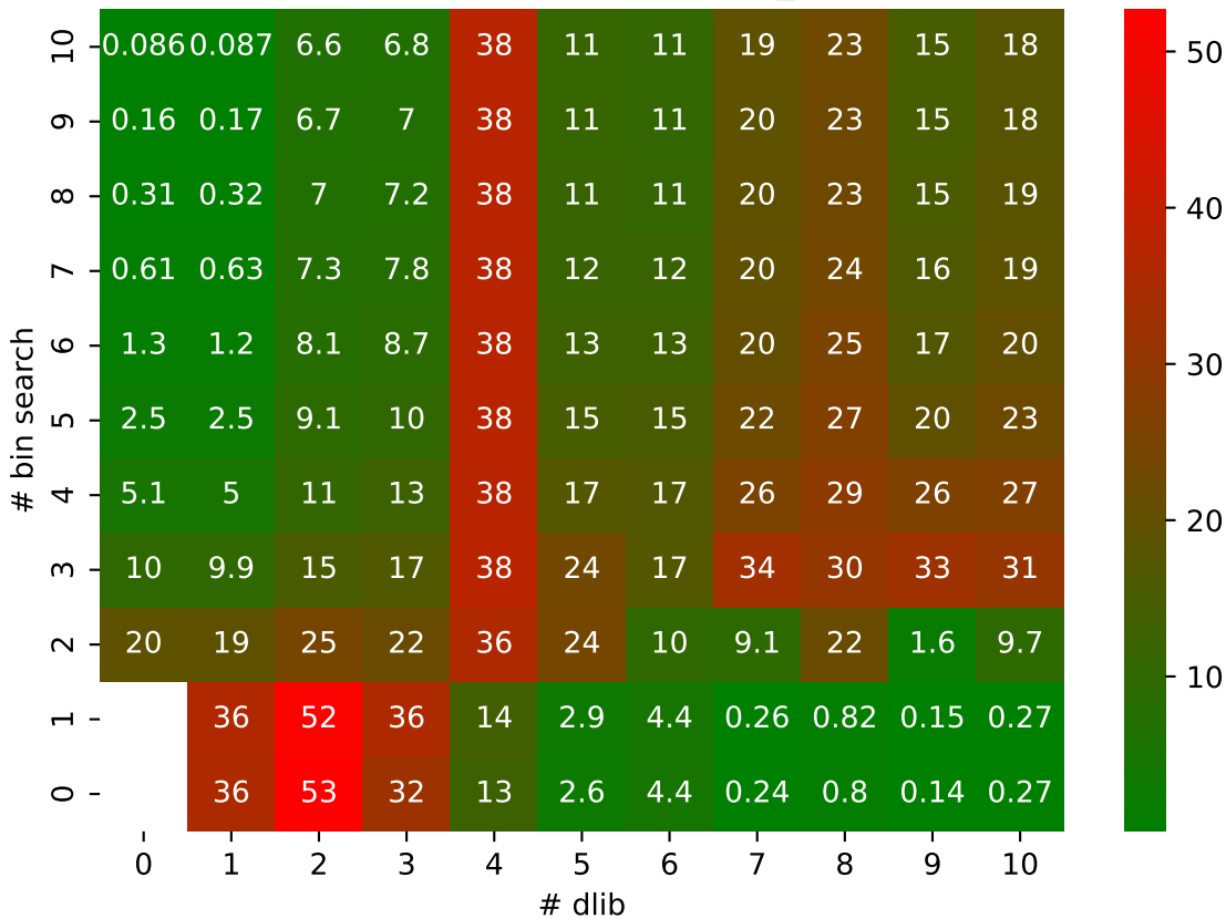
CLOUD SPERR pressio:abs MAPE: bin_search vs dlib
