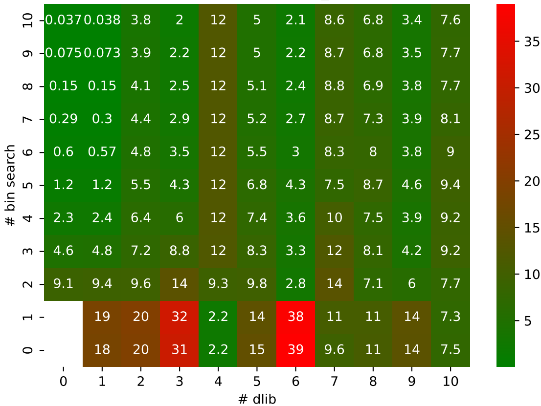
U SPERR pressio:abs MAPE: bin_search vs dlib
