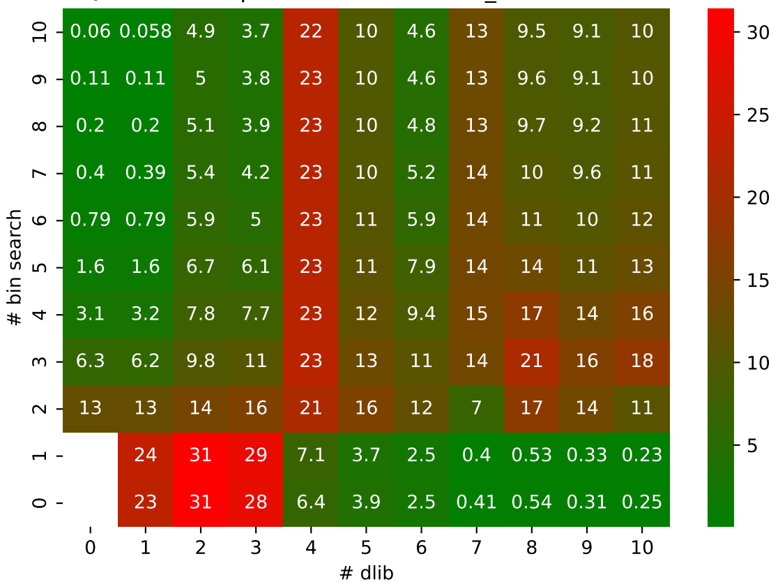
QRAIN SPERR pressio:abs MAPE: bin_search vs dlib
