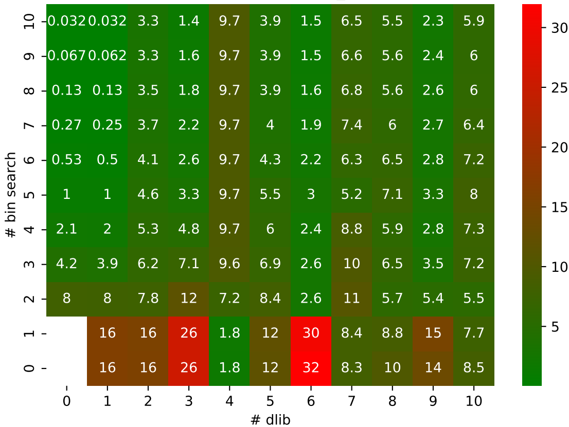
P SPERR pressio:abs MAPE: bin_search vs dlib
