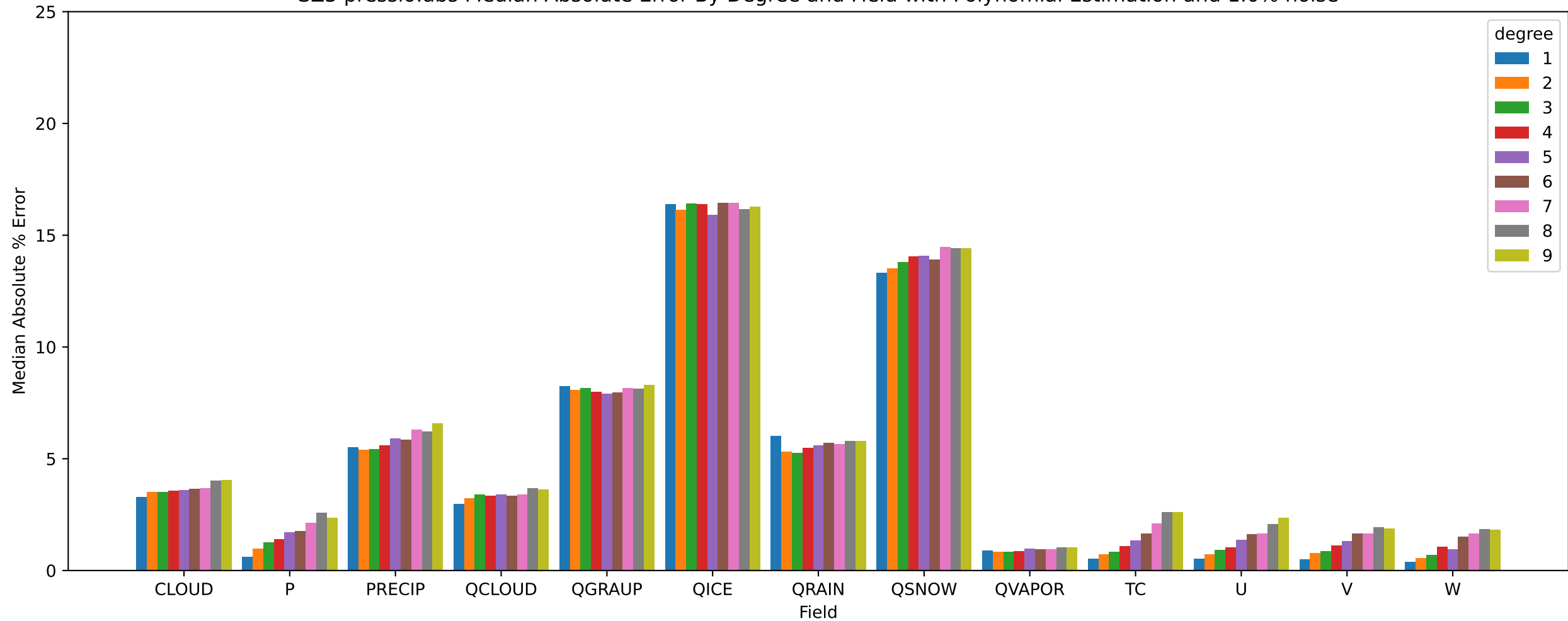
SZ3 pressio:abs Median Absolute Error By Degree and Field with Polynomial Estimation and 1.0% noise
