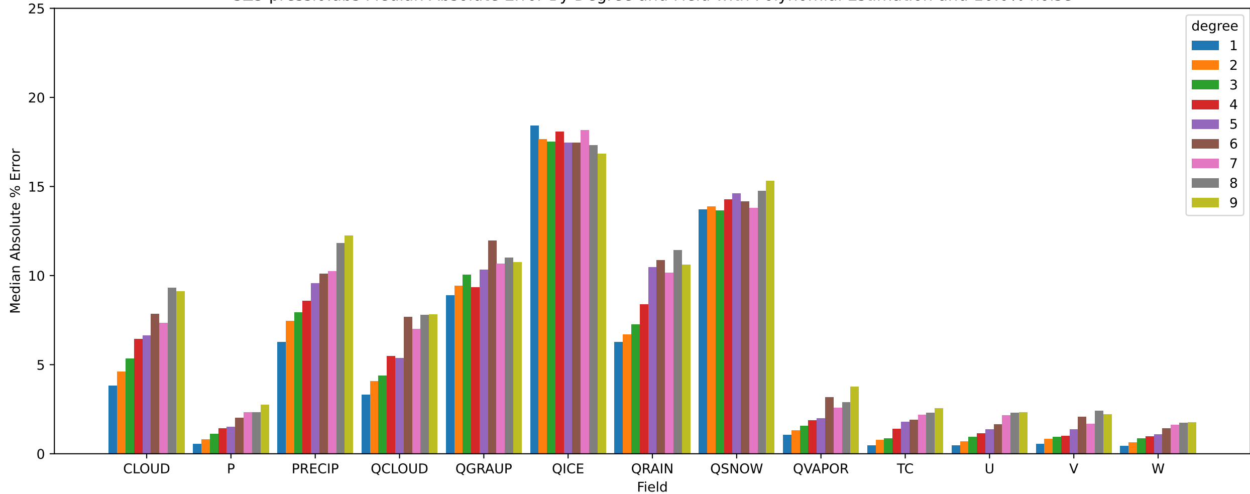
SZ3 pressio:abs Median Absolute Error By Degree and Field with Polynomial Estimation and 10.0% noise
